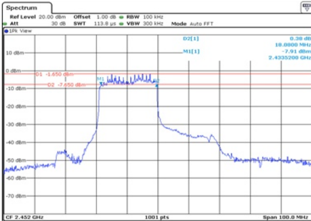
32 6 dB Bandwidth
