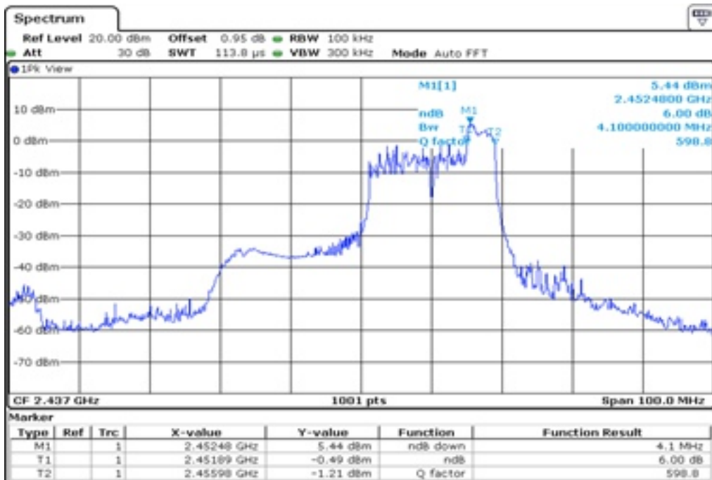
15 6 dB Bandwidth
