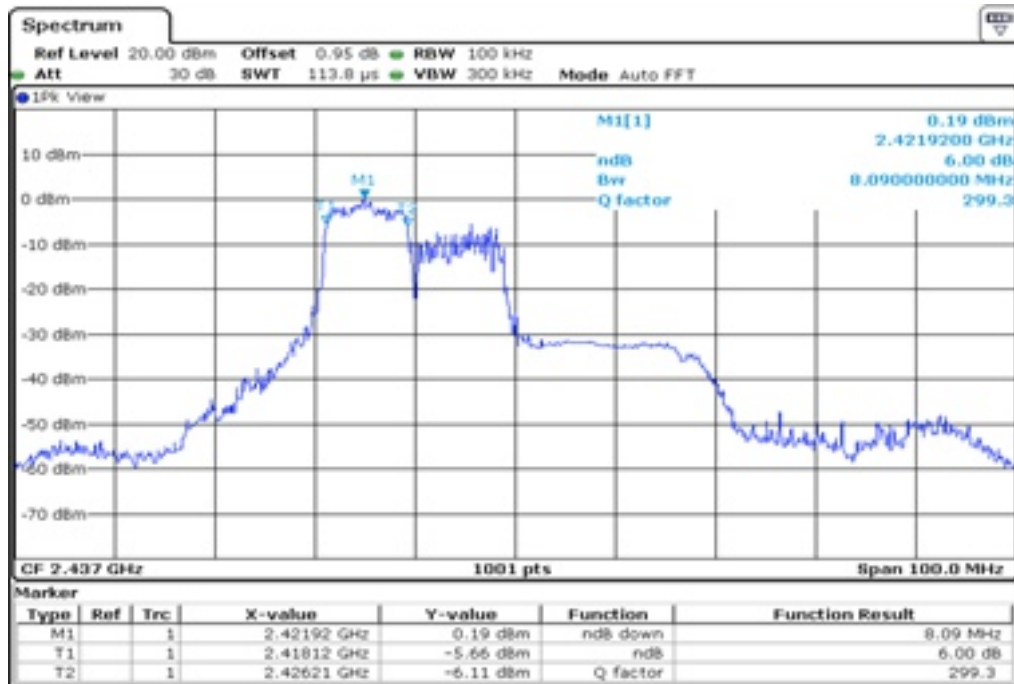
22 6 dB Bandwidth
