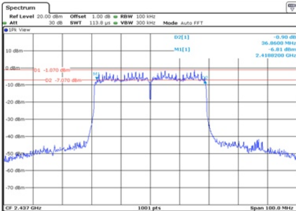
35 6 dB Bandwidth
