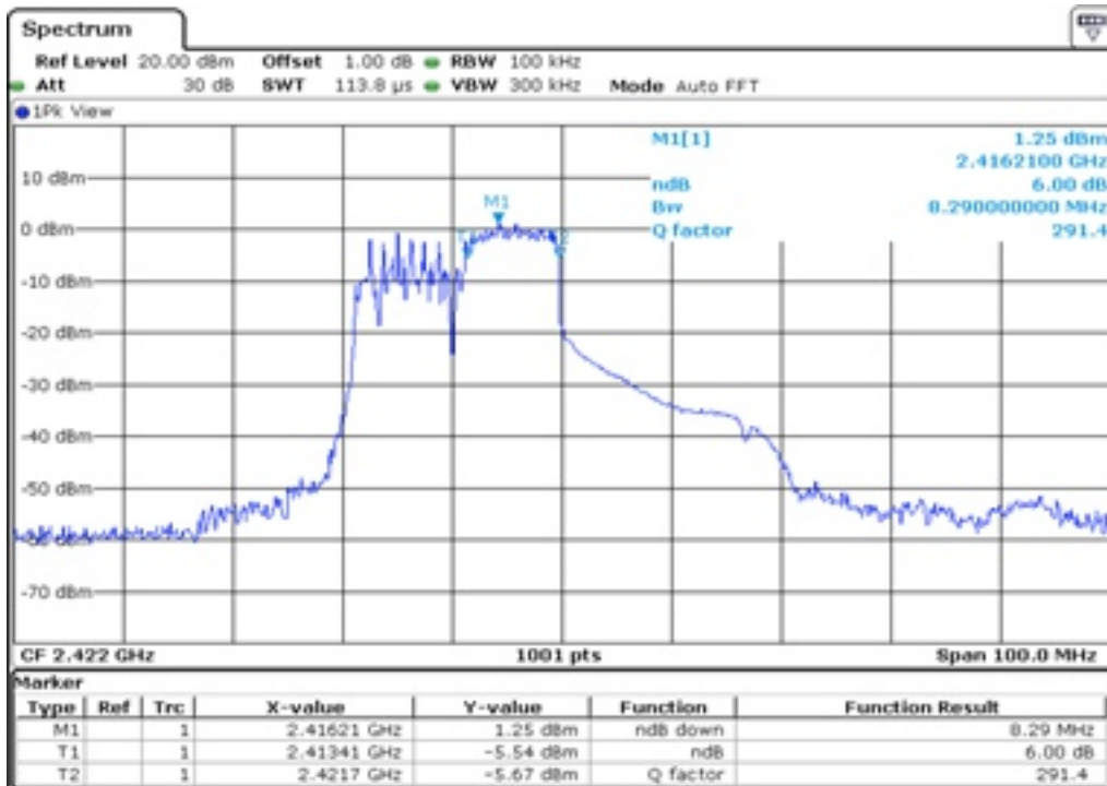
20 6 dB Bandwidth
