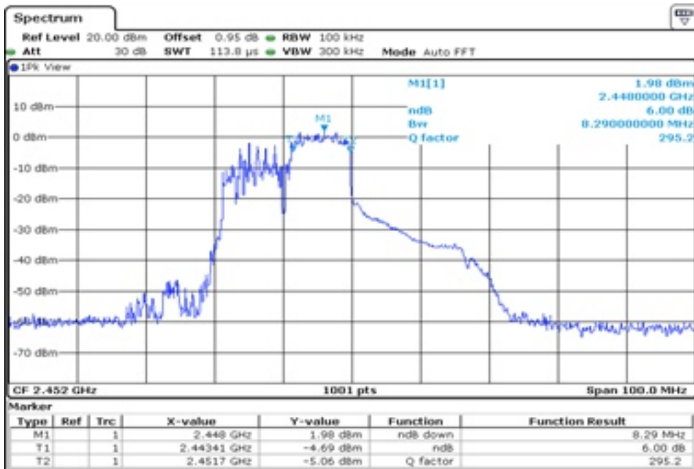
26 6 dB Bandwidth
