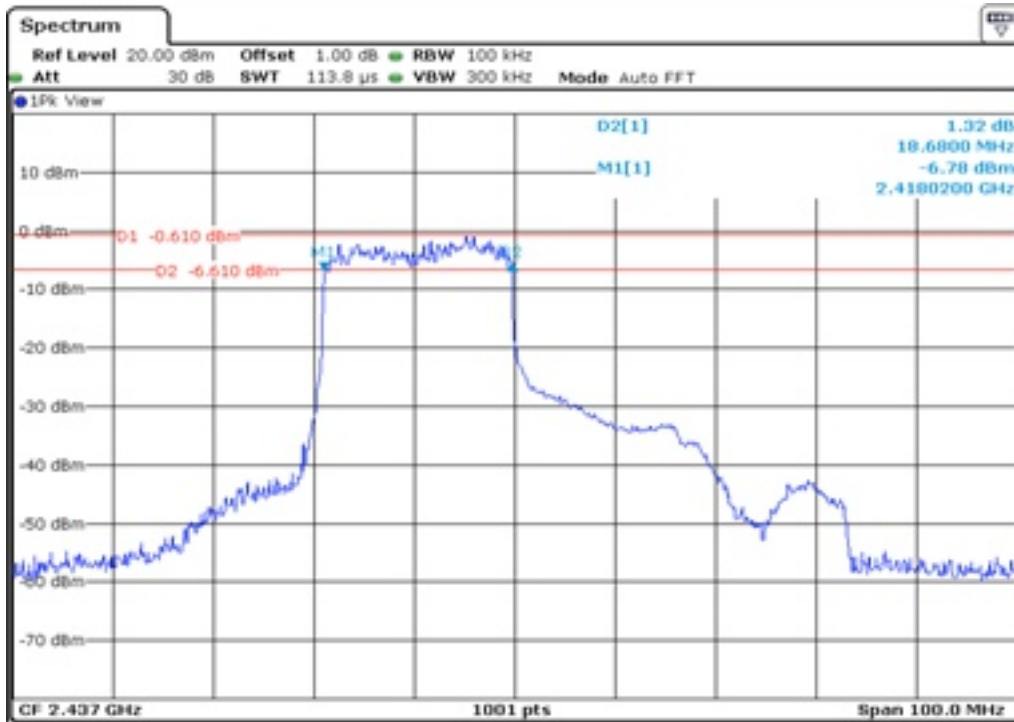
30 6 dB Bandwidth
