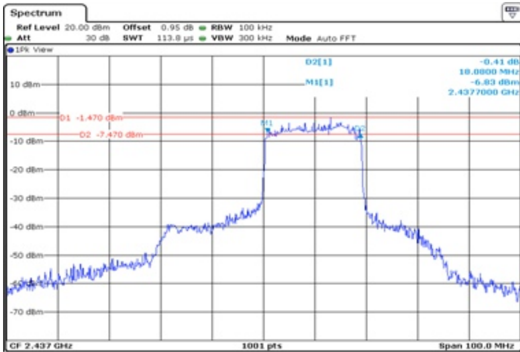
31 6 dB Bandwidth
