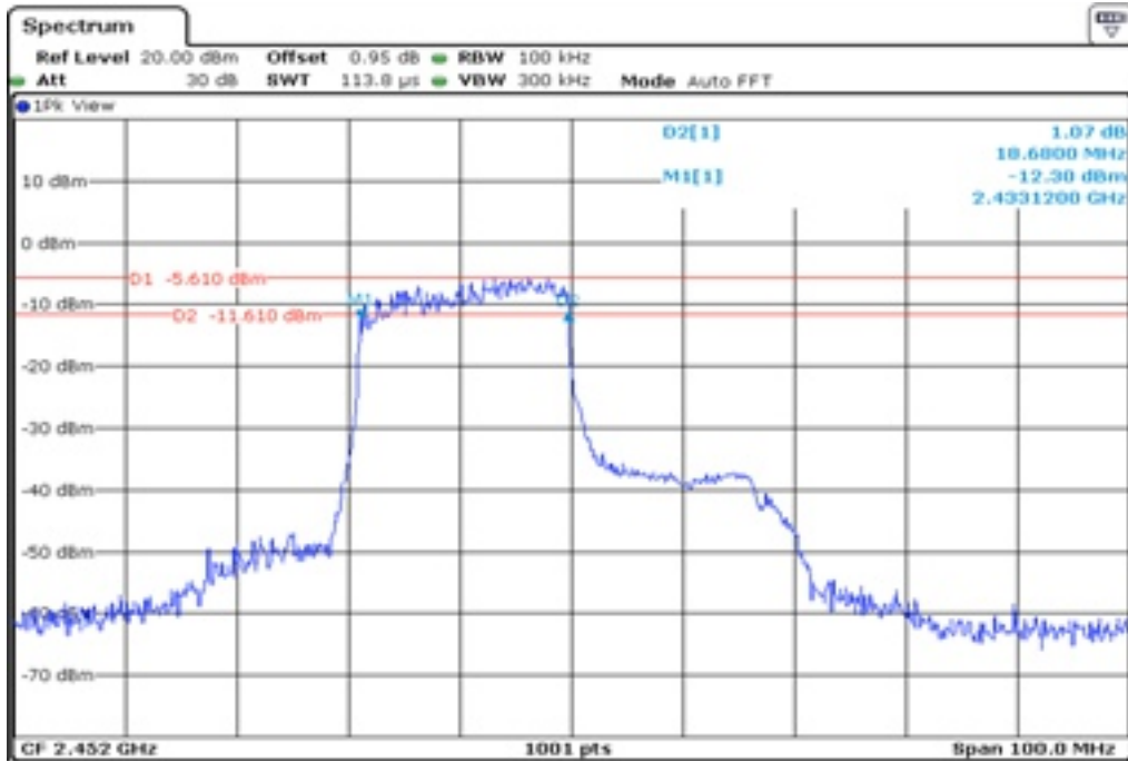
32 6 dB Bandwidth
