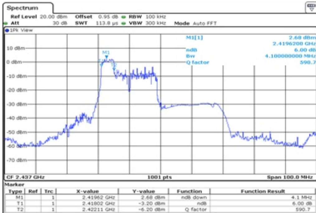
13 6 dB Bandwidth
