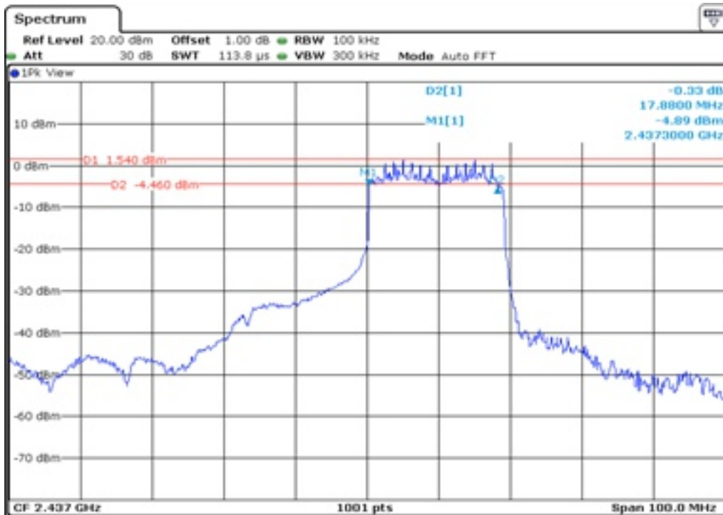
31 6 dB Bandwidth
