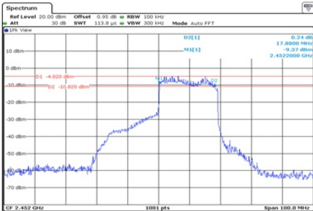
33 6 dB Bandwidth
