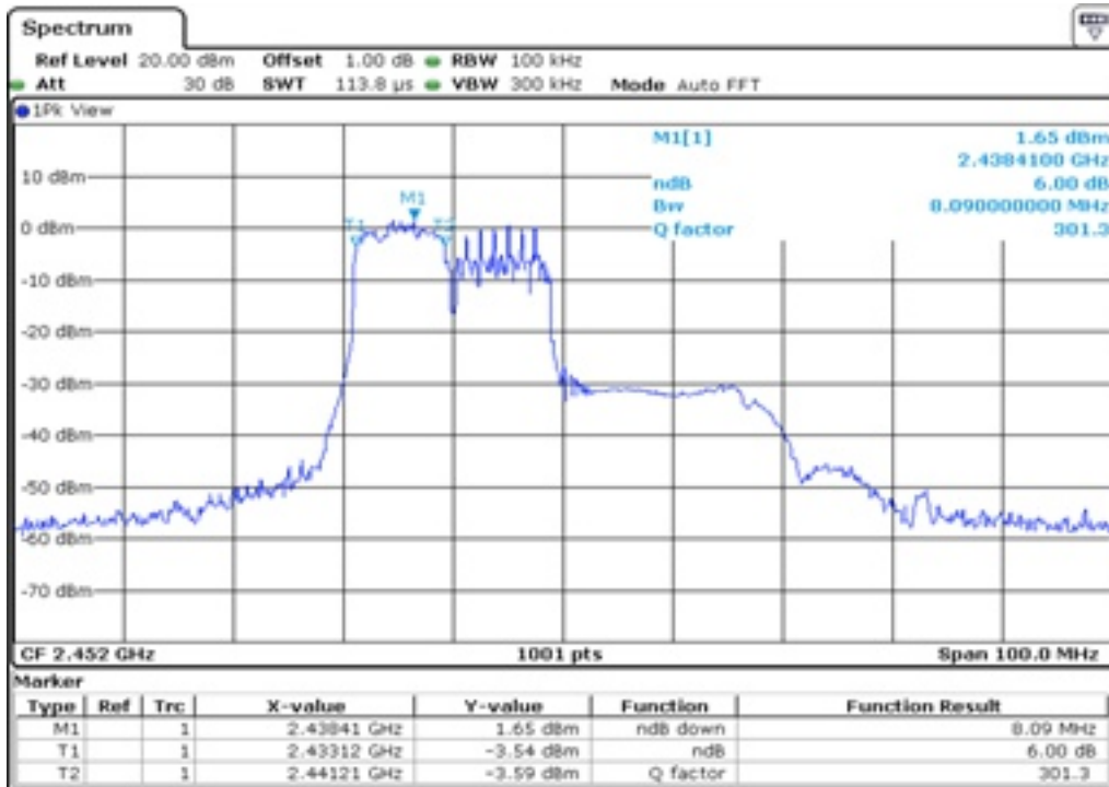
25 6 dB Bandwidth
