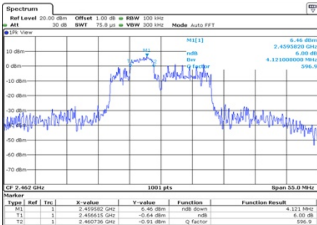
17 6 dB Bandwidth
