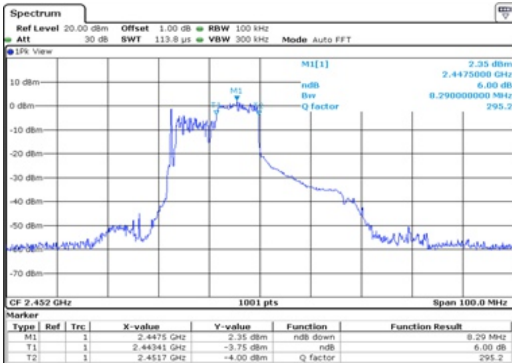
26 6 dB Bandwidth
