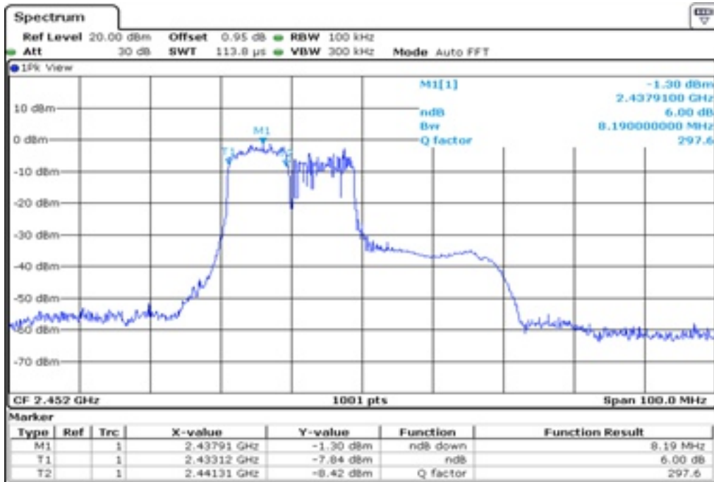
25 6 dB Bandwidth
