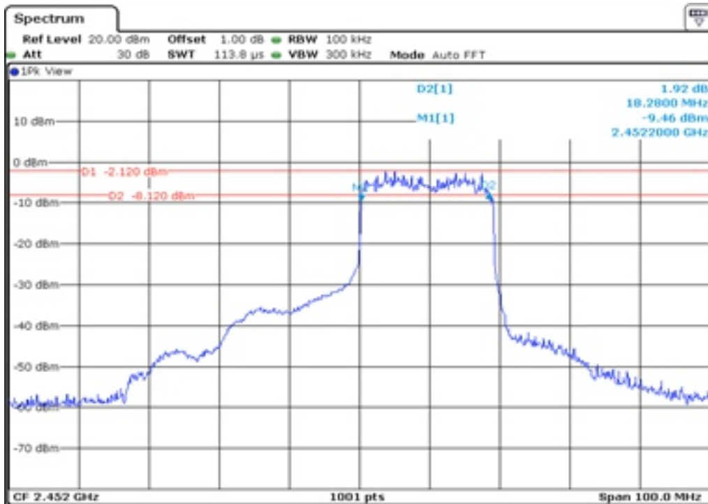
33 6 dB Bandwidth
