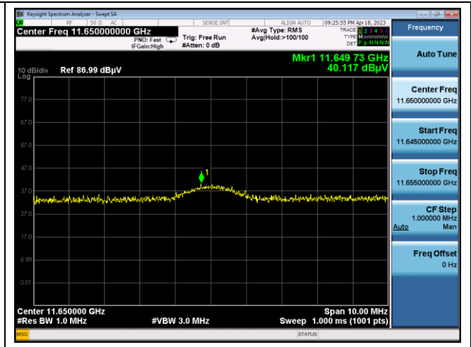
High channel 2 nd Spurious (Peak) - Band 3
