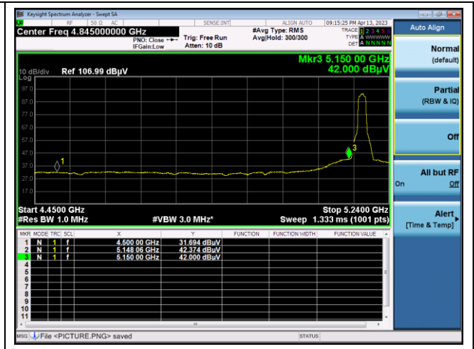
Middle channel 2 nd Spurious (Peak) - Band 1
