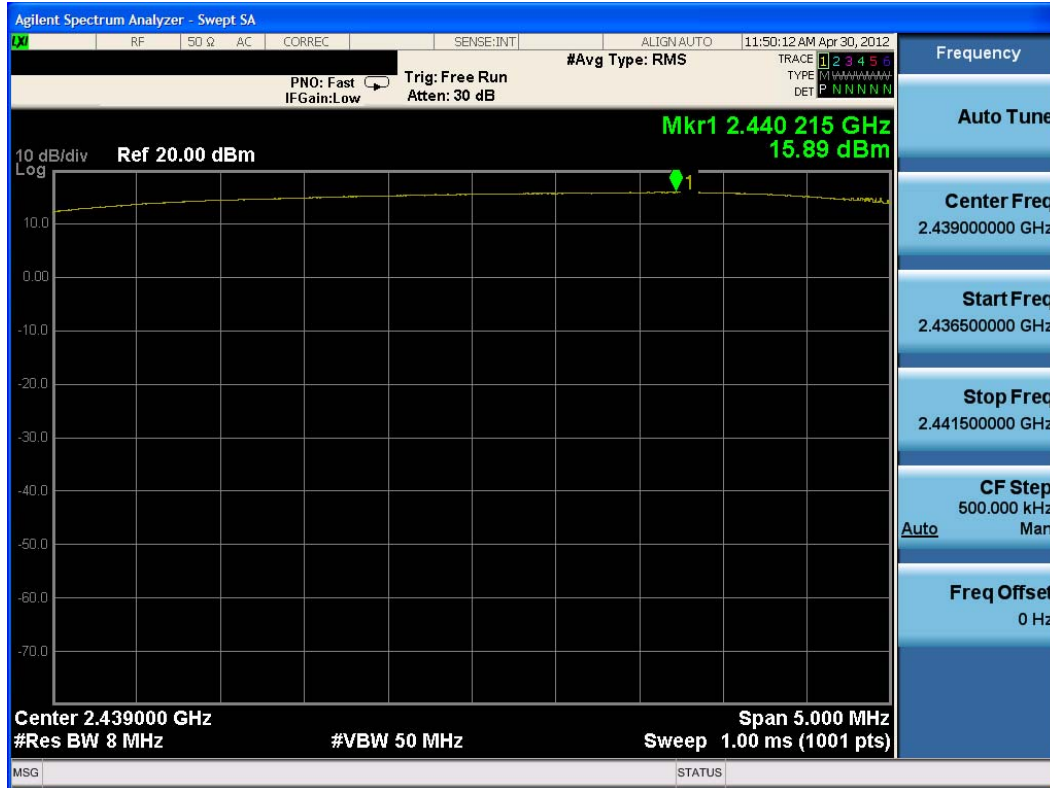
6-5. Conducted Power Plot (Mid Channel)
