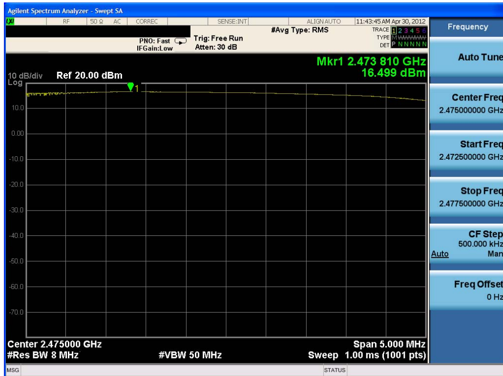
6-6. Conducted Power Plot (High Channel)
