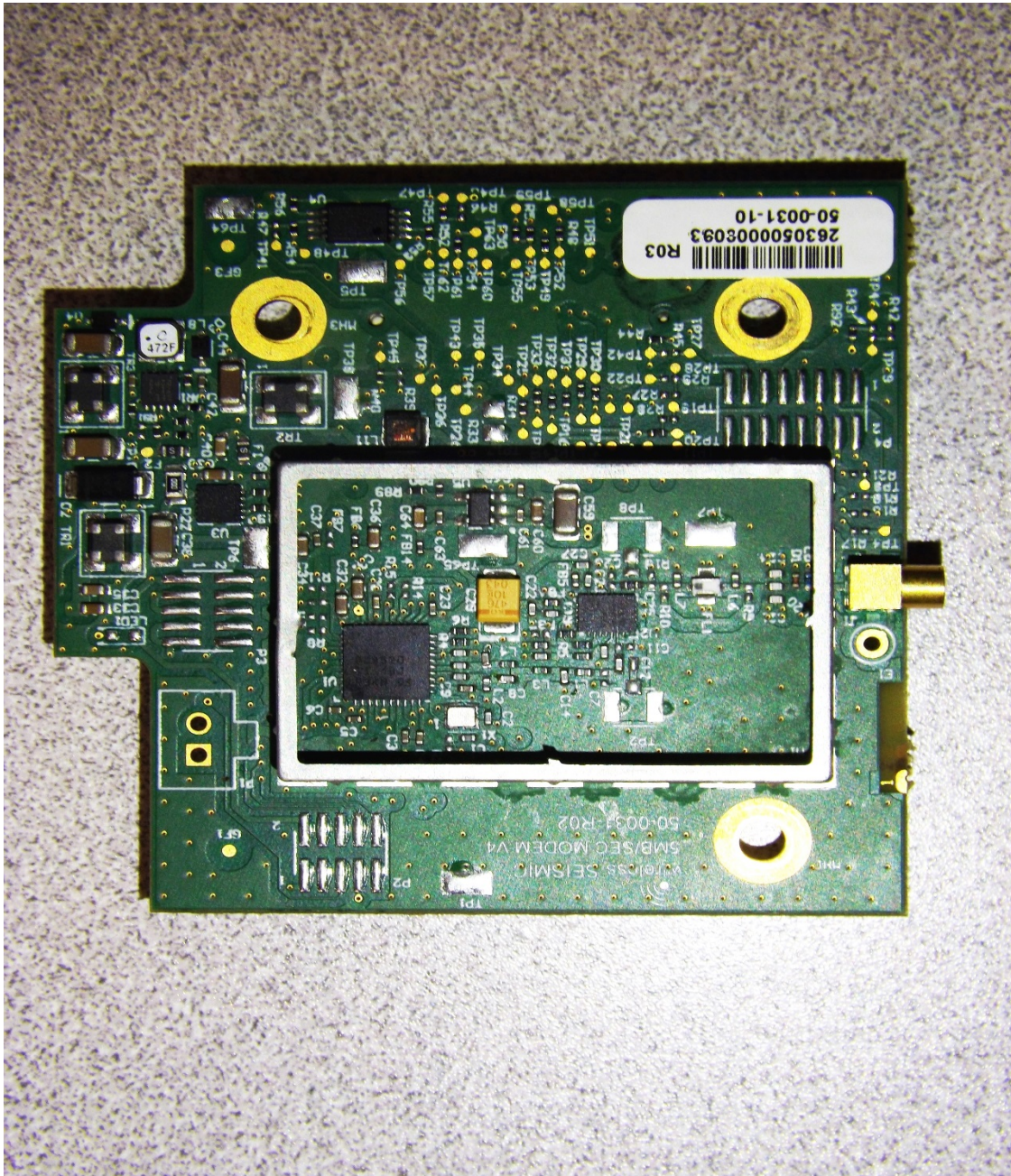
WRU, RF Modem Board, Model 50-0031 Topside (with RF Radio Shield removed)
