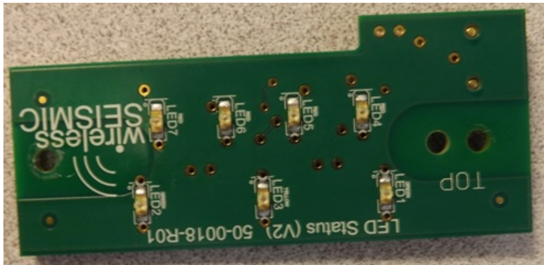
WRU, LED Board Model #50-0018 Topside
