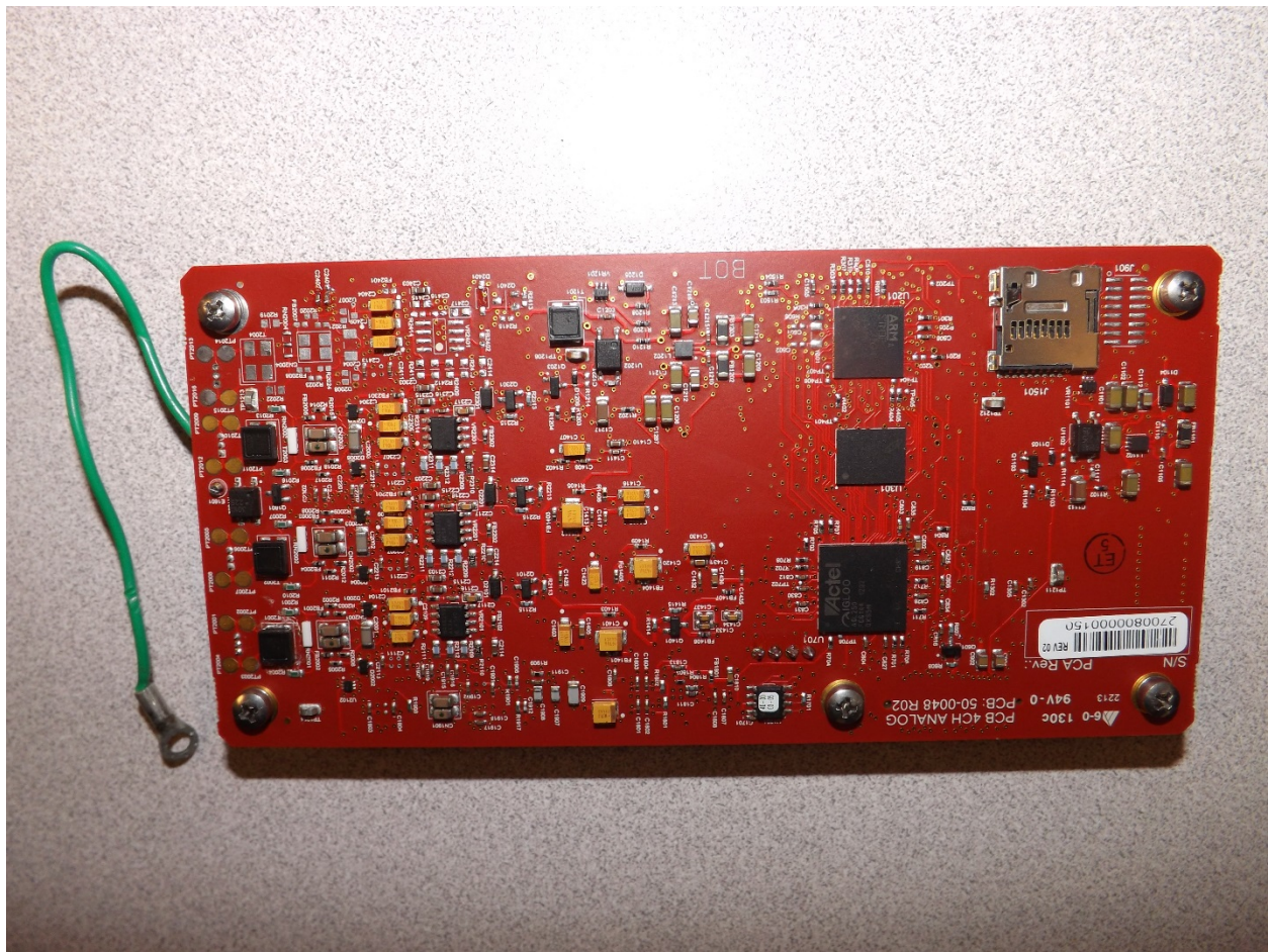
WRU, Analog Board, Model 50-0048 Underside
