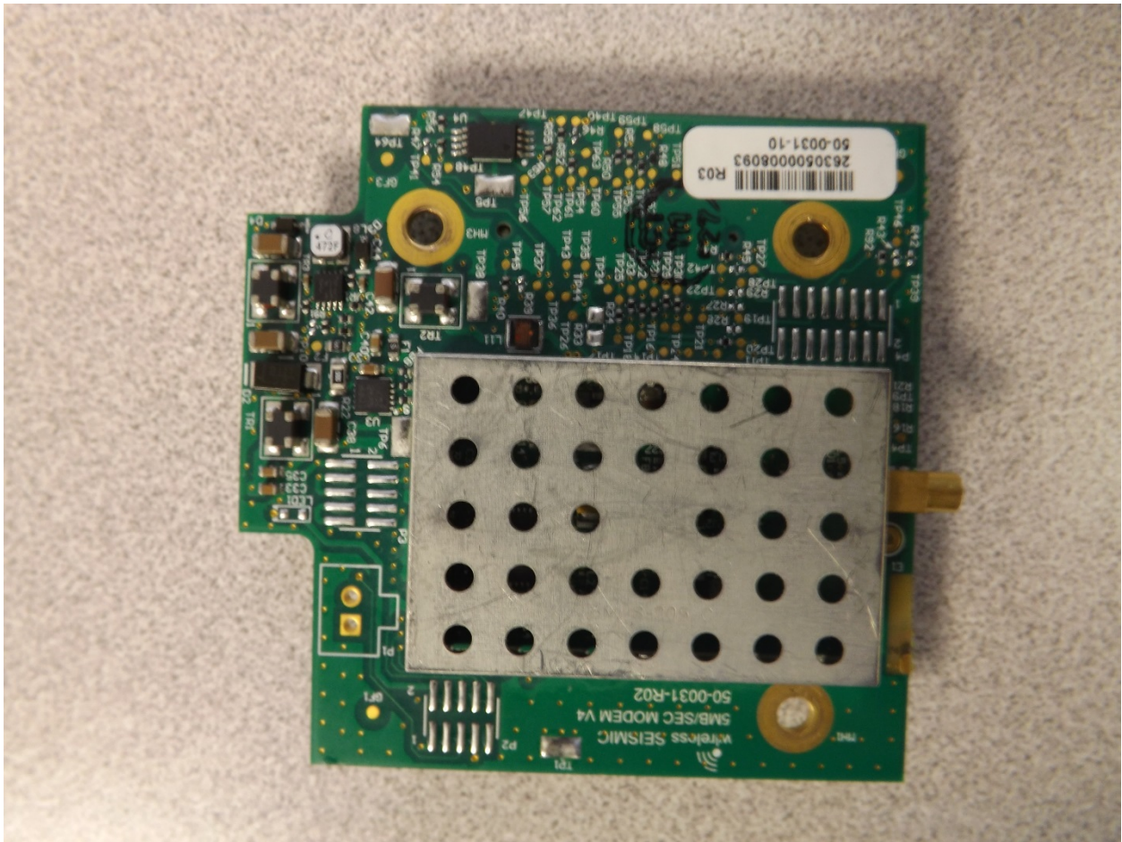
WRU, RF Modem Board, Model 50-0031 Topside
