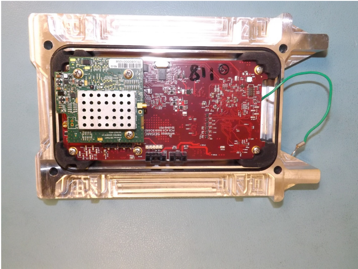
WRU, Model 10-0023 Overhead – Lower Enclosure (With PCB Stack, Model 15-0056)
