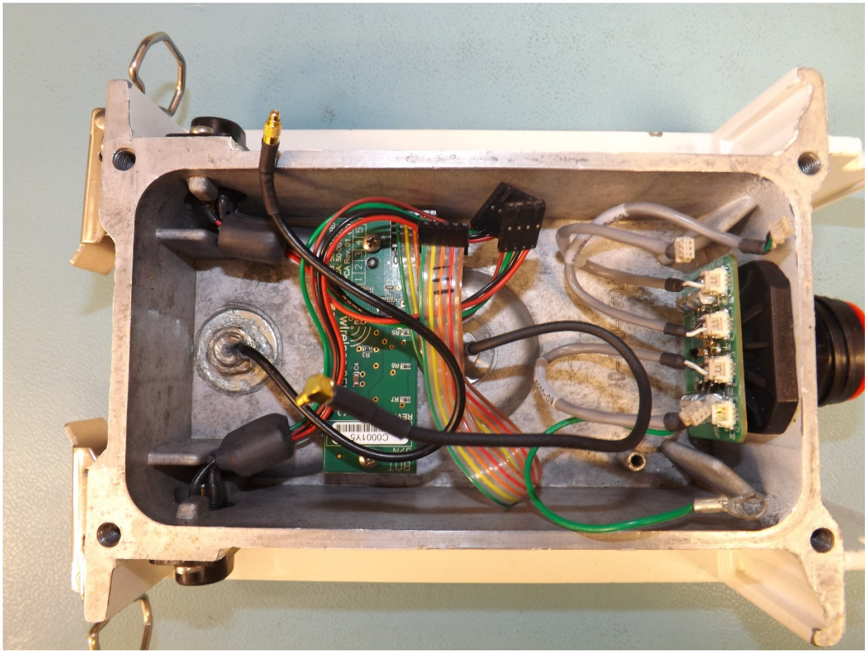
WRU, Model 10-0023 Overhead – Top Enclosure
