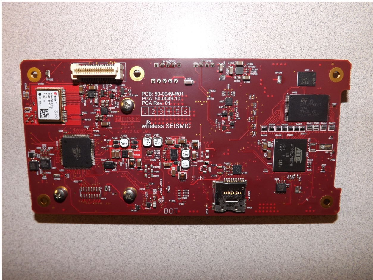
WRU, Main (Digital) Board, Model 50-0049 Underside
