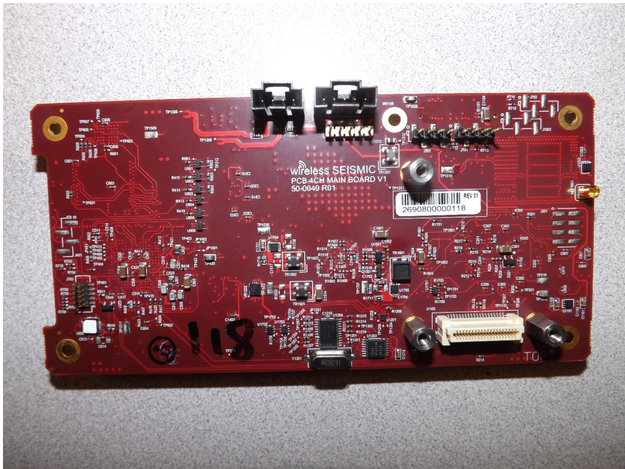
WRU, Main (Digital) Board, Model 50-0049 Topside
