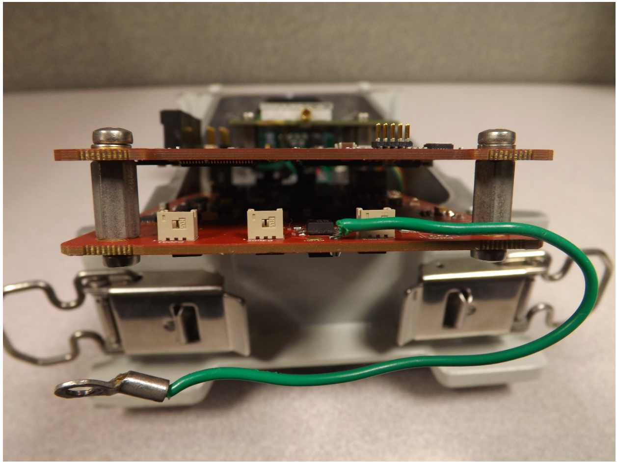
WRU, PCB Stack, Model 15-0056 Side
