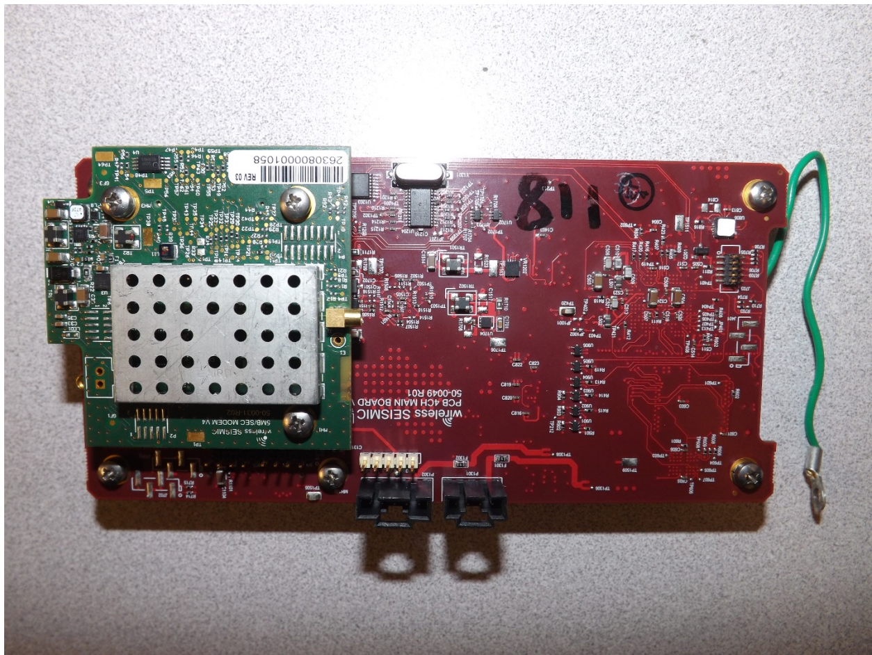
WRU, PCB Stack, Model 15-0056 Overhead
