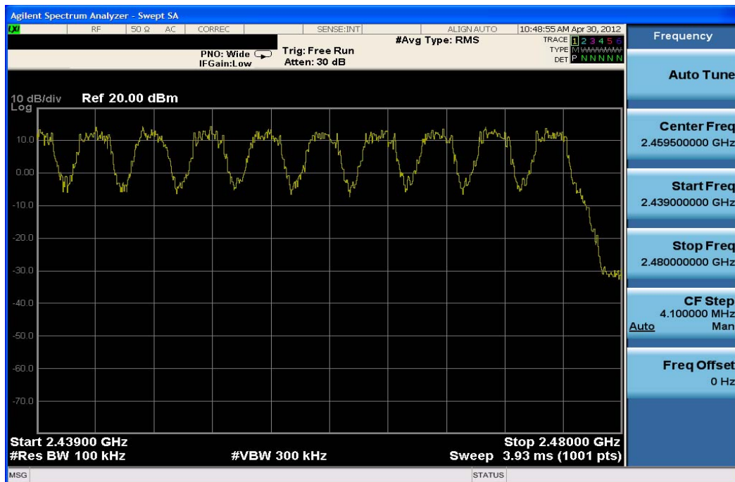
Plot 6-15. High End Spectrum Channel Hopping Plot
