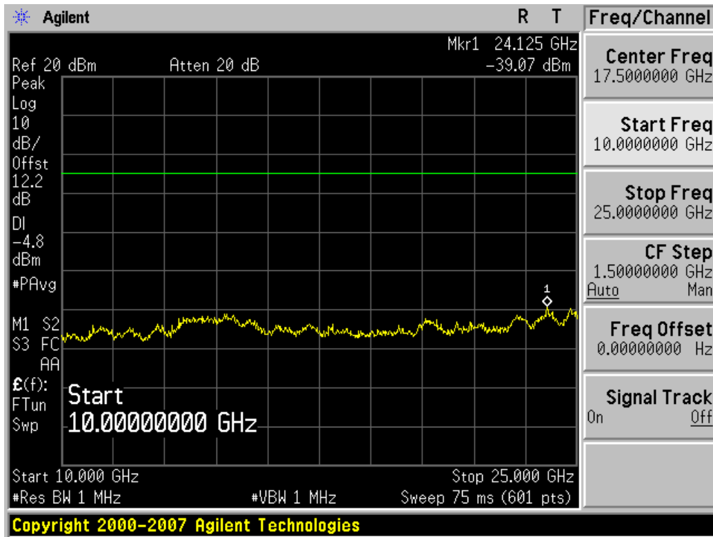
Plot 6-16. Conducted Spurious Plot (Ch. 16)
