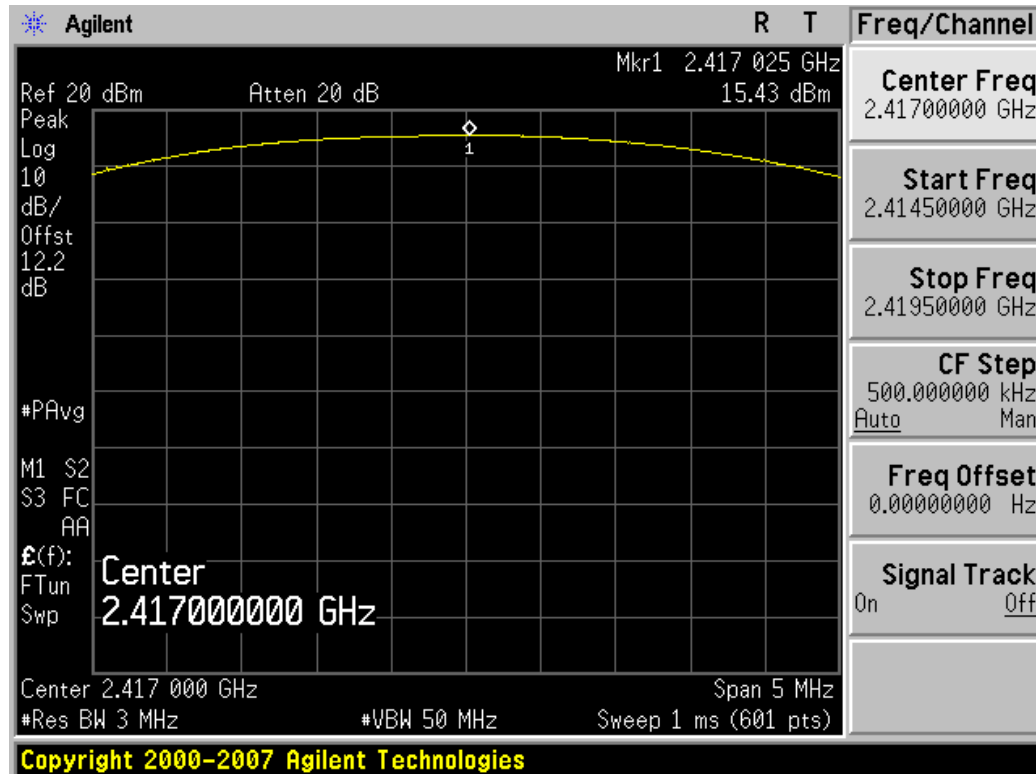
Plot 6-4. Peak Conducted Output Power Plot (Ch. 16)
