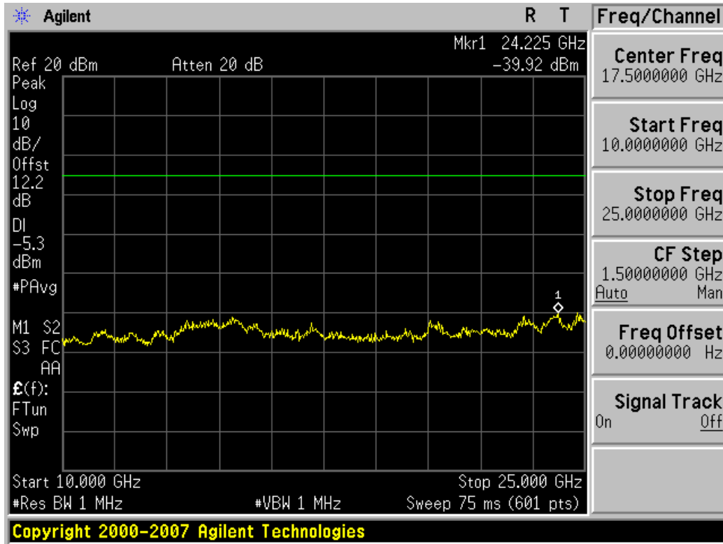
Plot 6-19. Conducted Spurious Plot (Ch. 42)
