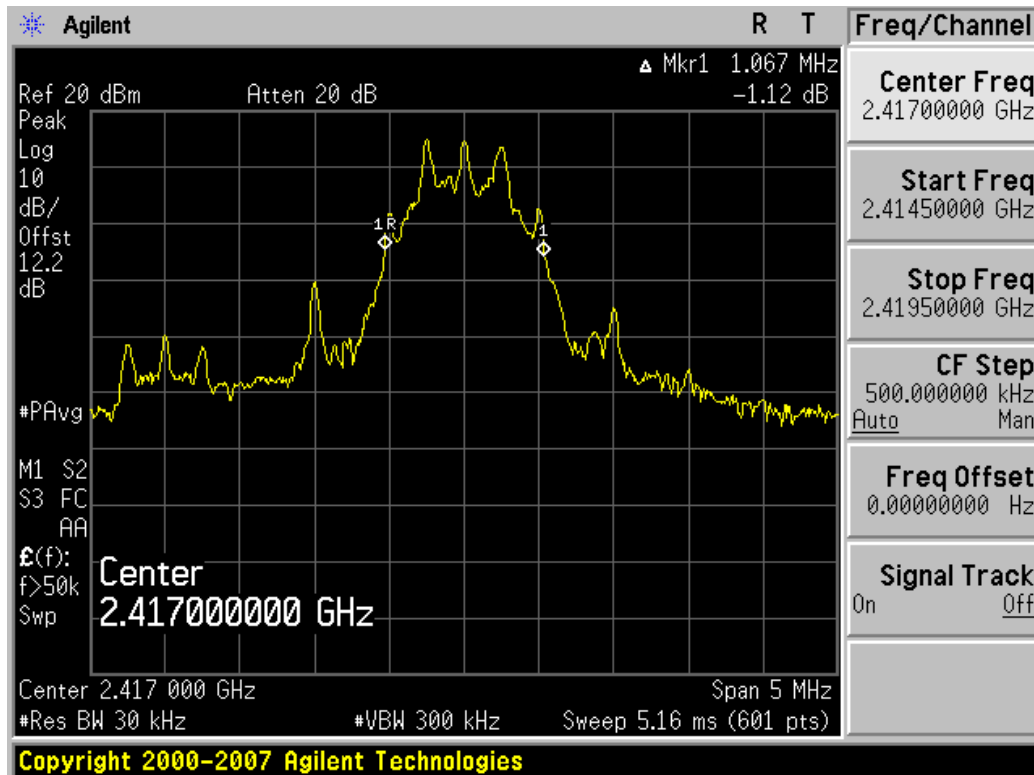
Plot 6-1. 20dB Bandwidth Plot (Ch. 16)
