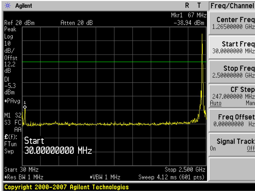
Plot 6-17. Conducted Spurious Plot (Ch. 42)
