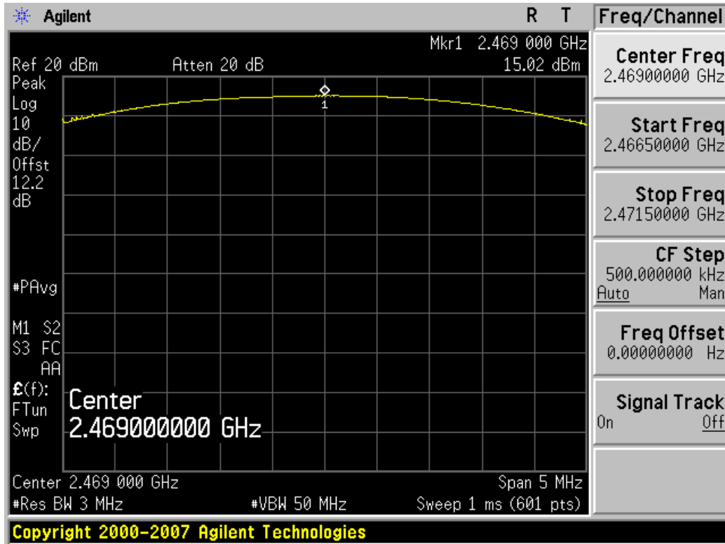
Plot 6-6. Peak Conducted Output Power Plot (Ch. 68)
