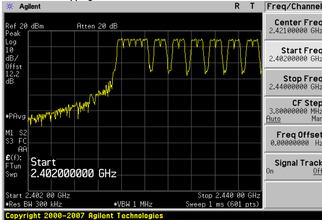
Plot 6-12. Low End Spectrum Channel Hopping Plot
