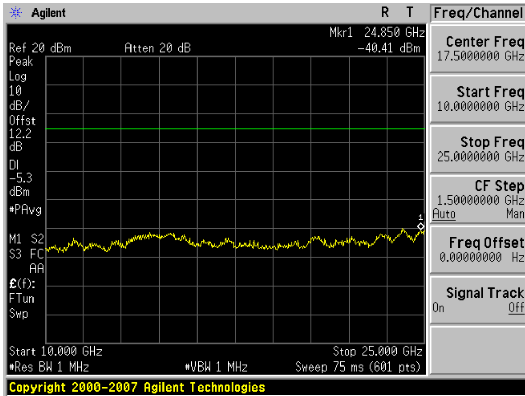
Plot 6-22. Conducted Spurious Plot (Ch. 68)
