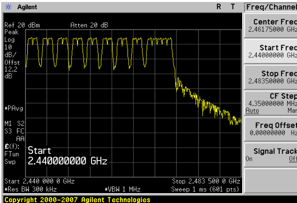
Plot 6-13. High End Spectrum Channel Hopping Plot
