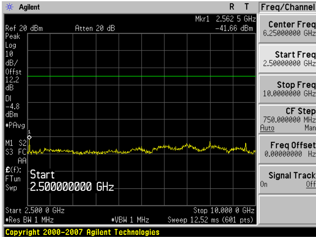
Plot 6-15. Conducted Spurious Plot (Ch. 16)
