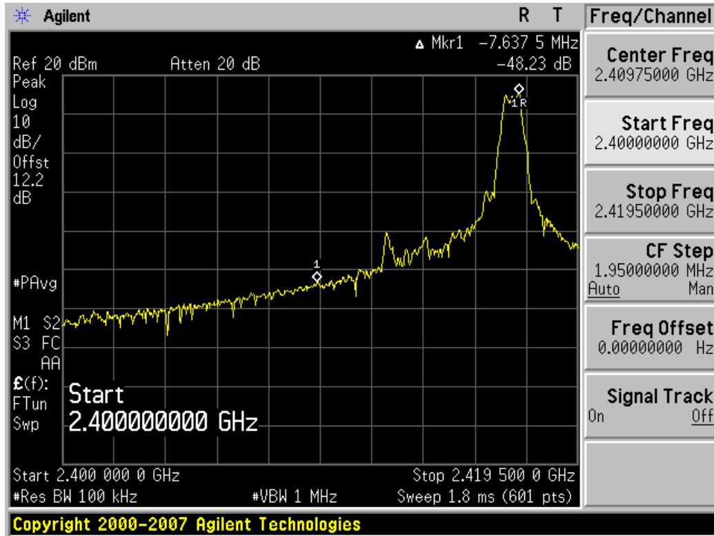
Plot 6-7. Lower Band Edge Plot (Ch. 16)
