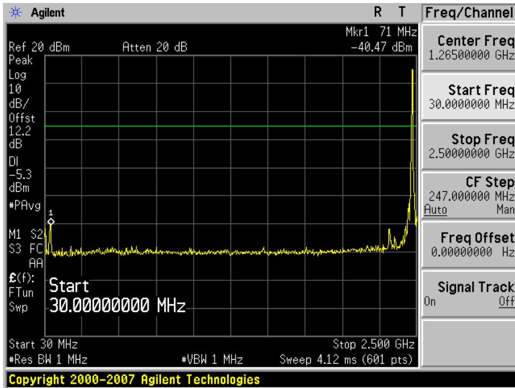
Plot 6-20. Conducted Spurious Plot (Ch. 68)
