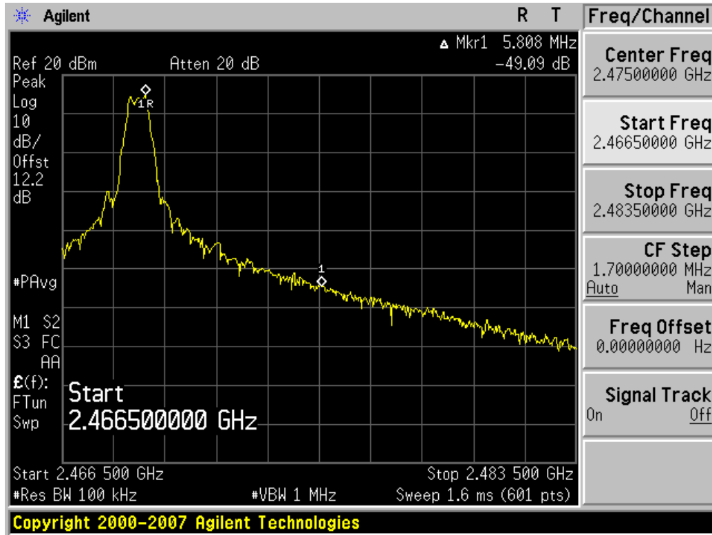
Plot 6-8. Upper Band Edge Plot (Ch. 68)
