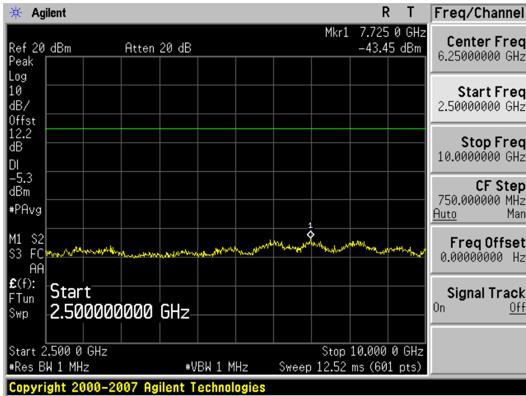
Plot 6-18. Conducted Spurious Plot (Ch. 42)
