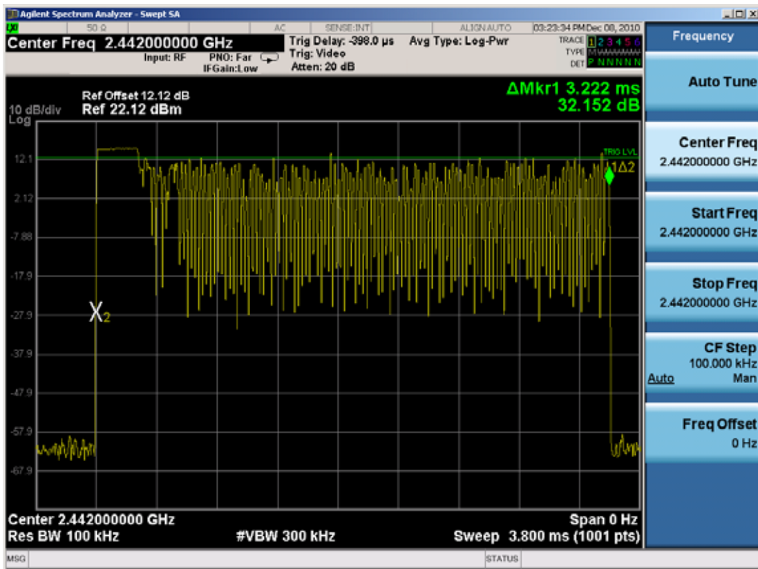
Plot 6-10. Time of Occupancy Plot
