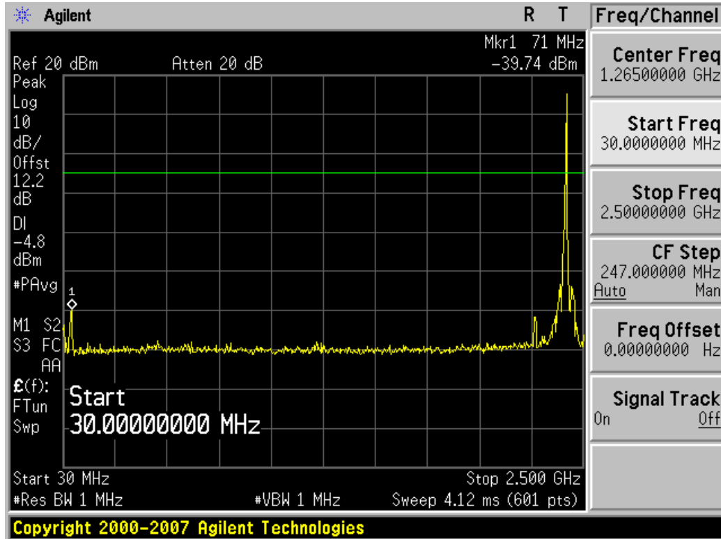
Plot 6-14. Conducted Spurious Plot (Ch. 16)
