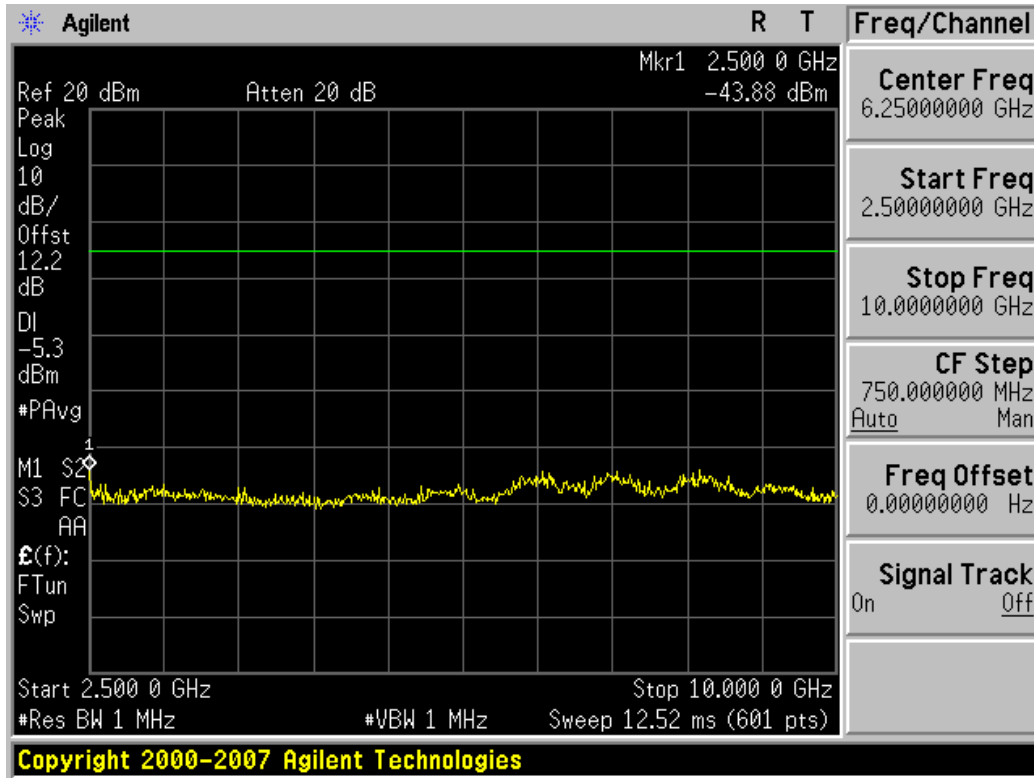
Plot 6-21. Conducted Spurious Plot (Ch. 68)
