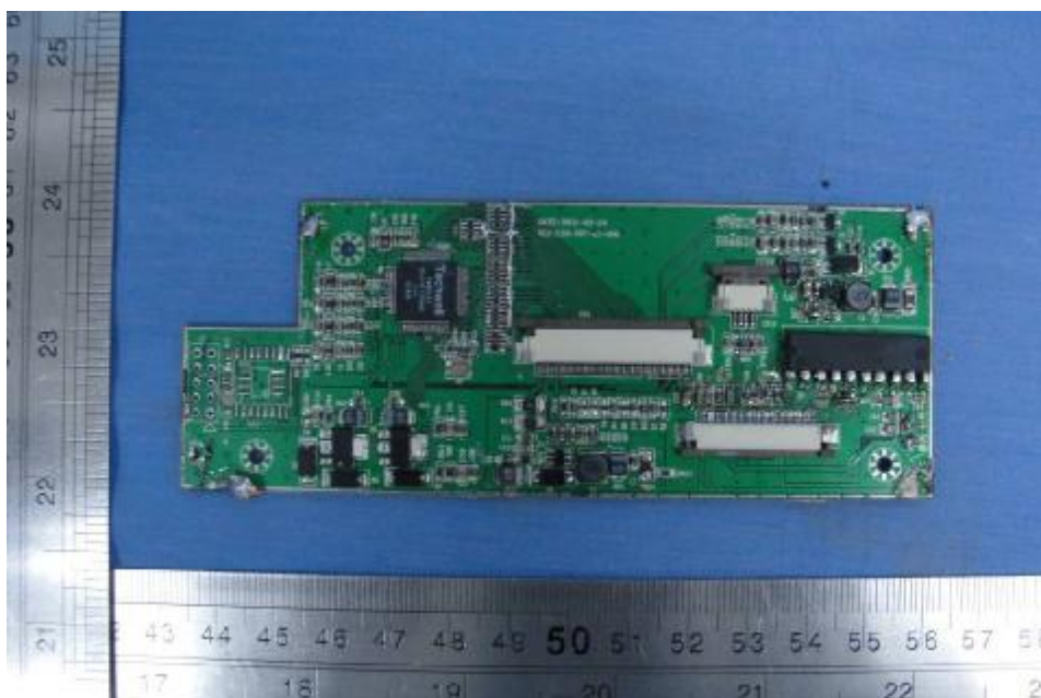
Internal View of EUT-8
