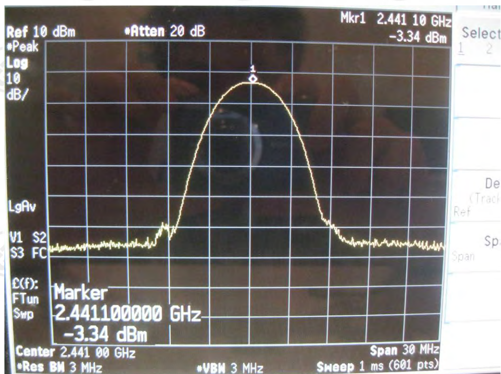
2441MHz
