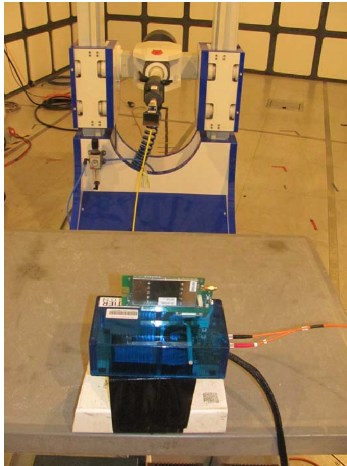
Radiated Emissions 18GHz-40GHz– PIFA Antenna
