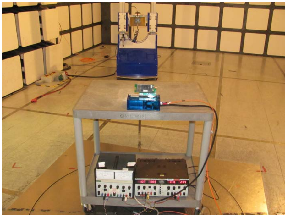
Radiated Emissions 30MHz-1GHz – PIFA Antenna
