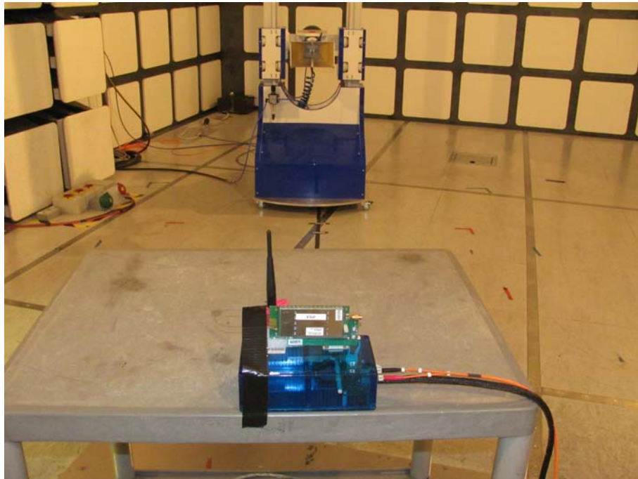
Radiated Emissions 1GHz-18GHz– External Antenna
