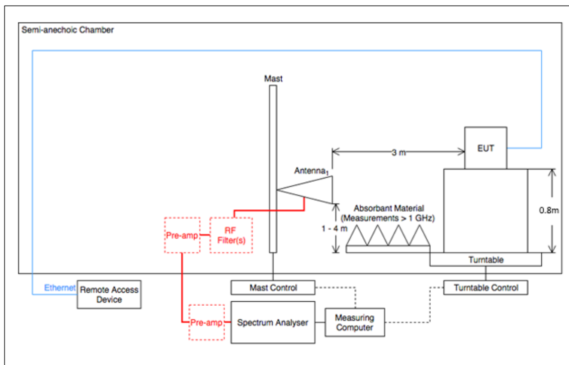
Figure 8 - Radiated Disturbance Example Test Setup
