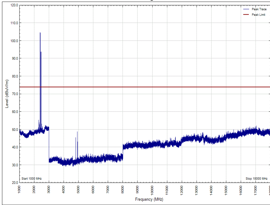
Figure 30 - 1 GHz to 18 GHz - Y Orientation - Peak, Polarisation: Vertical
