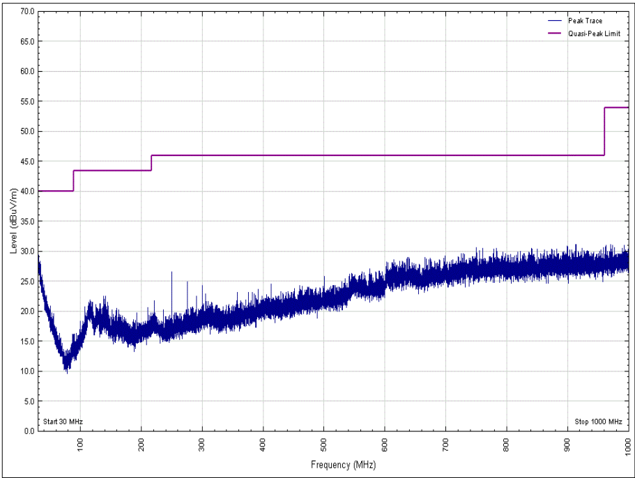
Figure 62 - 30 MHz to 1 GHz, 2480 MHz, Polarity: Horizontal, EUT Orientation X
