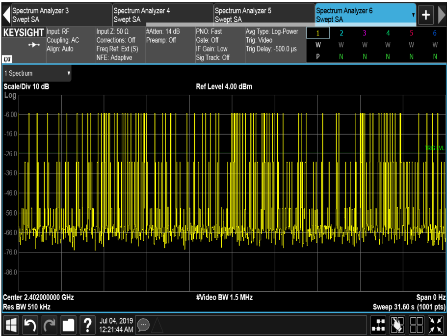
Figure 17 - DH5, Total Average Time of Occupancy
