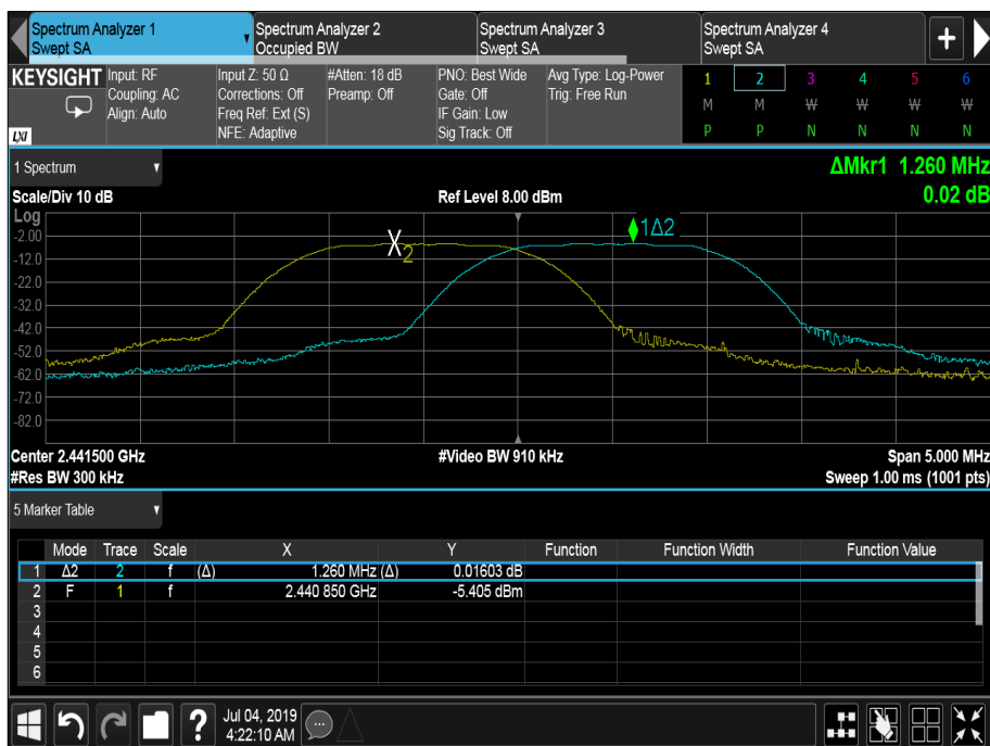
Figure 14 - \pi/4 DQPSK
