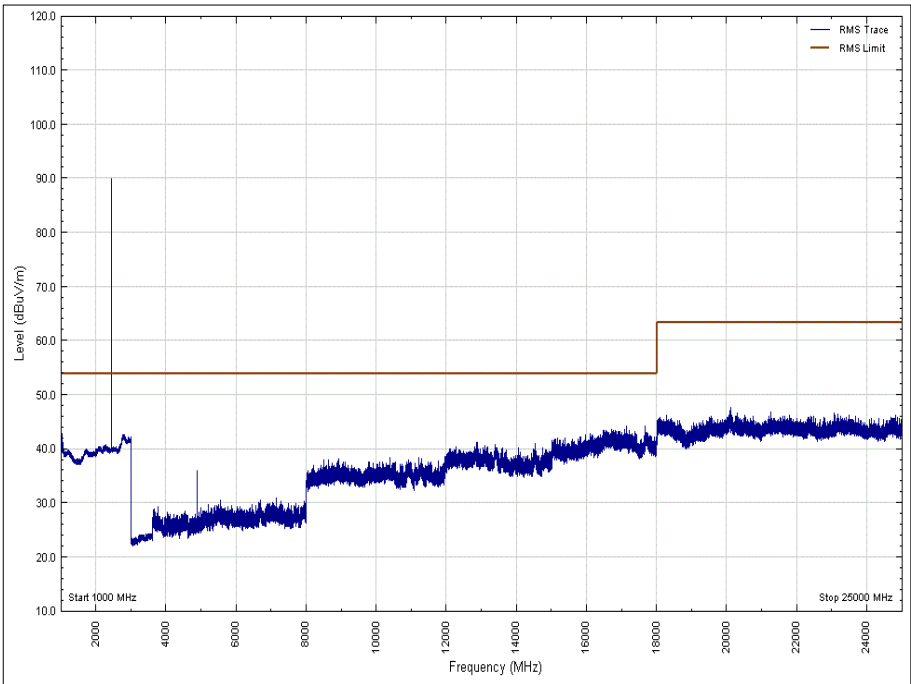
Figure 50 - 2441 MHz - 1 GHz to 25 GHz, Polarity: Vertical, EUT Orientation: X, Average
