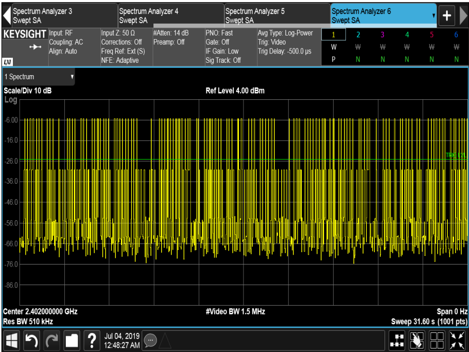
Figure 19 - DH3, Total Average Time of Occupancy
