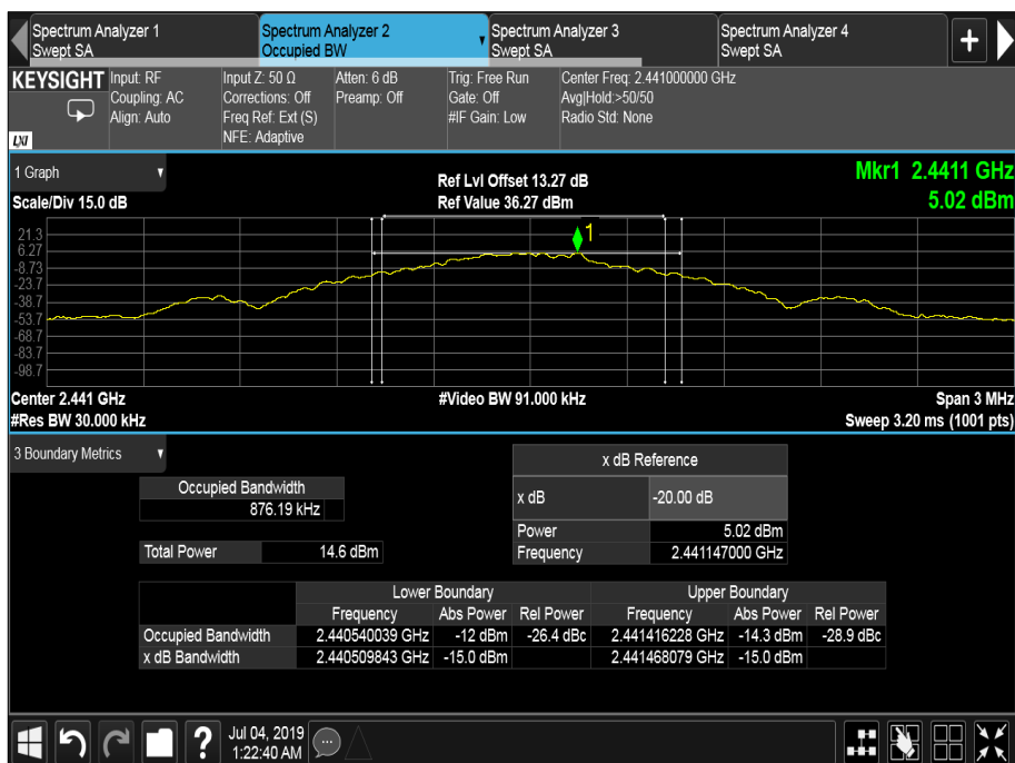
Figure 6 - 2441 MHz - GFSK
