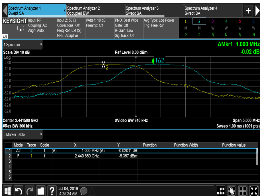
Figure 15 - 8-DPSK
