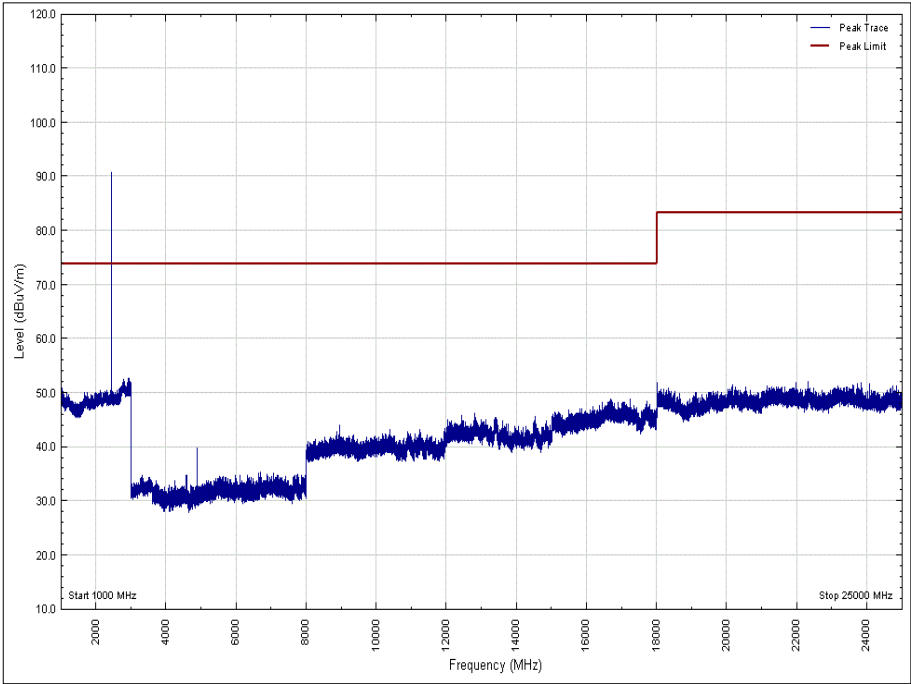
Figure 49 - 2441 MHz - 1 GHz to 25 GHz, Polarity: Vertical, EUT Orientation: X, Peak
