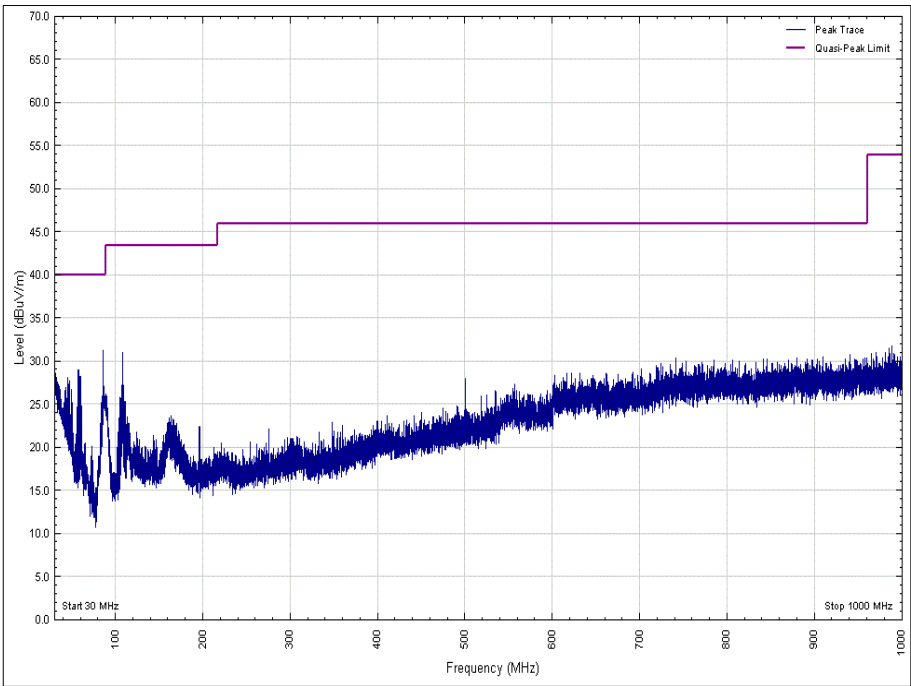
Figure 61 - 30 MHz to 1 GHz, 2480 MHz, Polarity: Vertical, EUT Orientation X
