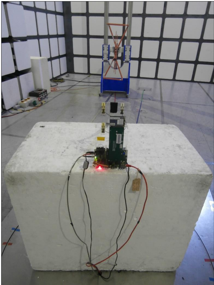
Figure 39 - 30 MHz to 1 GHz - Y Orientation
