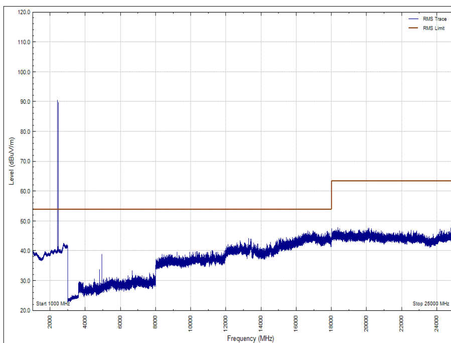
Figure 27 - 1 GHz to 25 GHz - X Orientation - Average, Polarisation: Vertical
