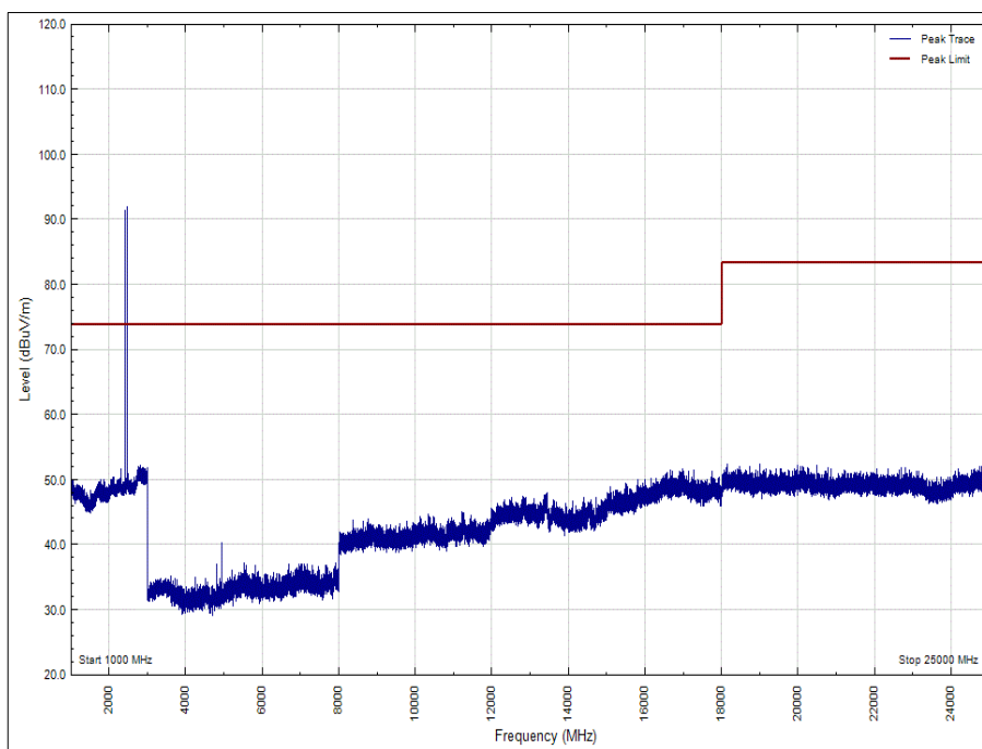
Figure 26 - 1 GHz to 25 GHz - X Orientation - Peak, Polarisation: Vertical
