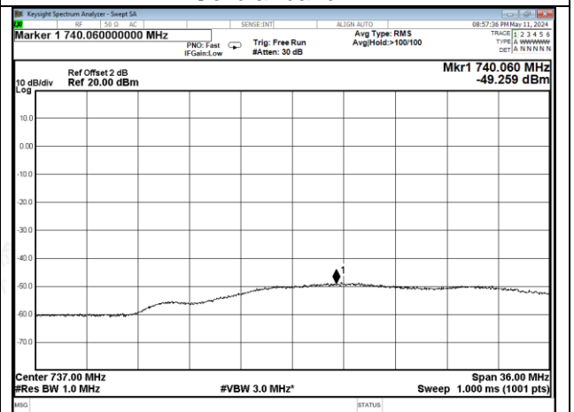
Lower 700MHz band DL
