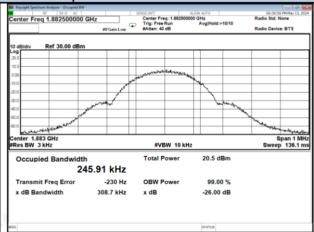
GSM-PCS band UL output
