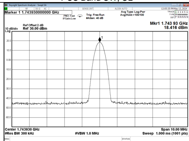
AWS Band CW, UL
