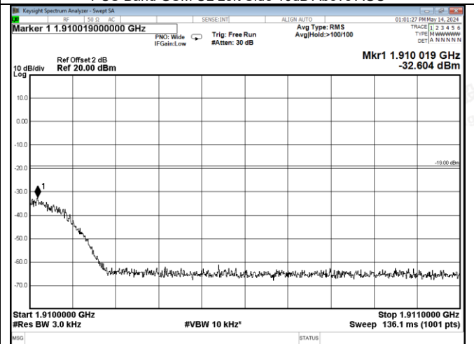
PCS Band GSM UL Right Side 10dB Above AGC
