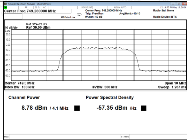
Upper 700MHz Band AWGN, DL
