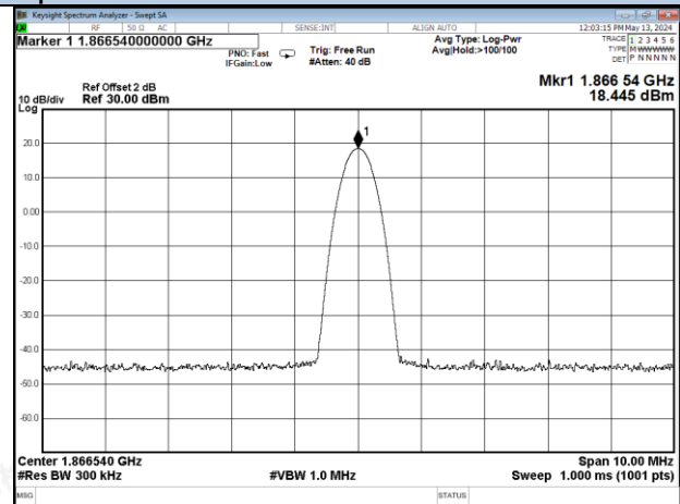
PCS Band CW, UL
