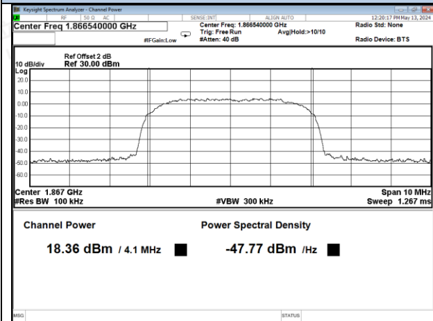
PCS Band AWGN, UL
