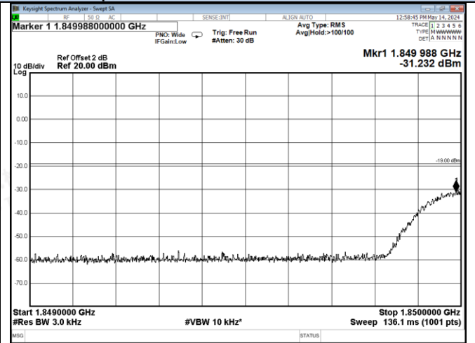
PCS Band GSM UL Left Side 10dB Above AGC
