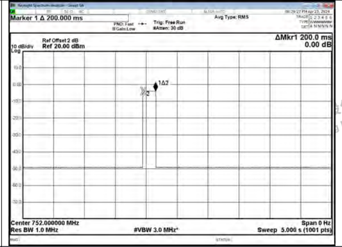
Detection Time-Upper 700 Band DL
