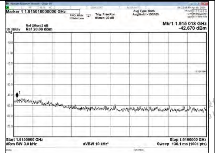
PCS Band UL-CDMA Right Side AGC+10dB
