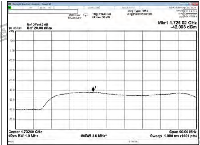
AWS Band UL
