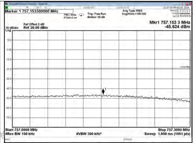
Upper 700 Band DL-CDMA Right Side AGC+10dB
