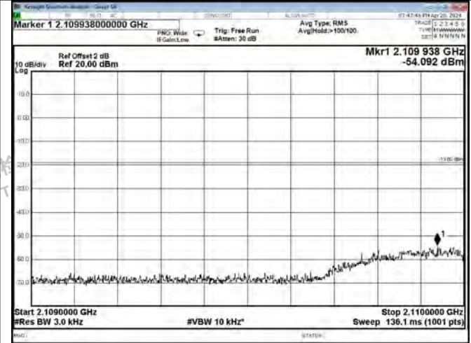
AWS Band DL-CDMA Left Side AGC+10dB
