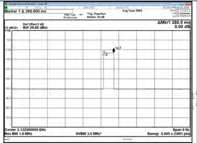
Detection Time-AWS Band DL
