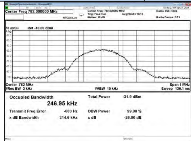
GSM-Upper 700 Band UL Input
