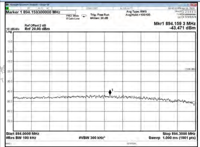
Cellular Band DL-CDMA Right Side AGC+10dB
