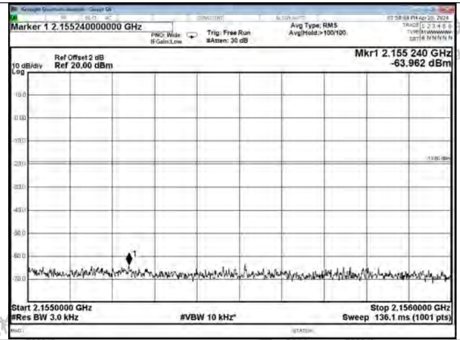
AWS Band DL-LTE Right Side AGC+10dB
