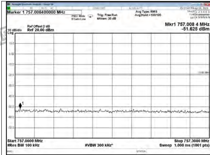
Upper 700 Band DL-LTE Right Side Pre AGC
