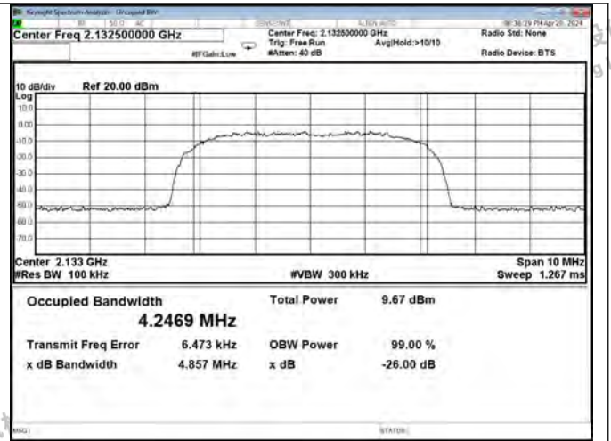
LTE-AWS Band DL Output
