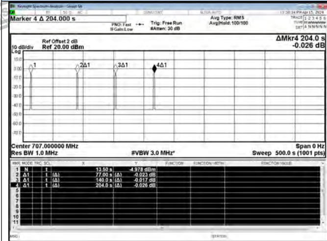
Restarting Time-Lower 700 Band UL
