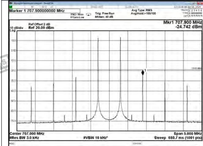
Lower 700 Band Pre AGC, UL
