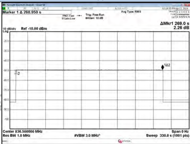
Cellular Band
