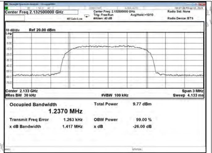
CDMA-AWS Band DL Output
