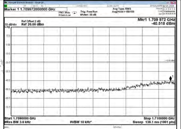
AWS Band UL-CDMA Left Side AGC+10dB
