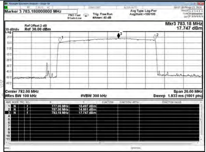
Upper 700 Band
