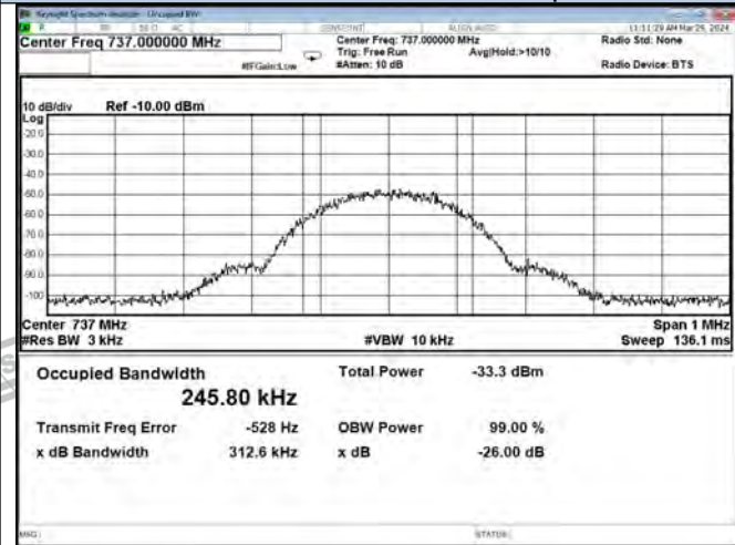
GSM-Lower 700 Band DL Input
