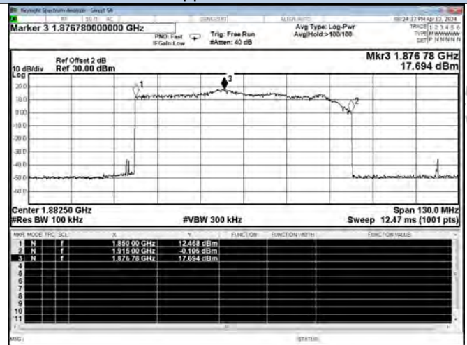
PCS Band
