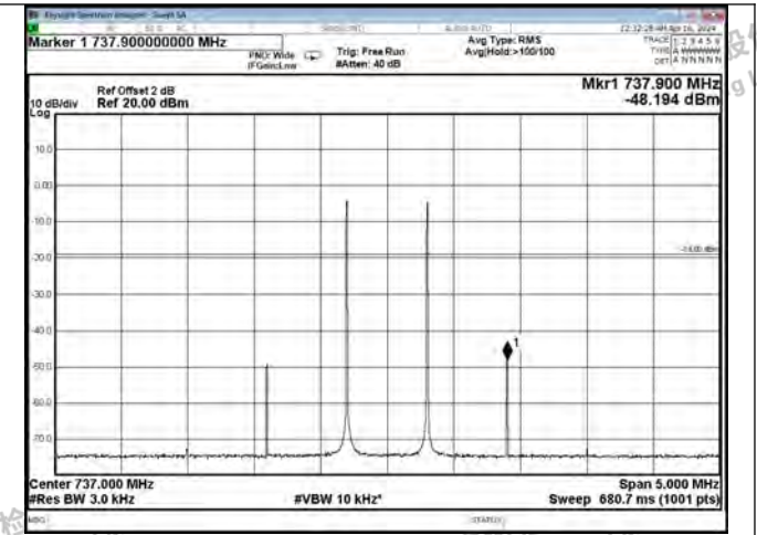
Lower 700 Band AGC+10dB, DL
