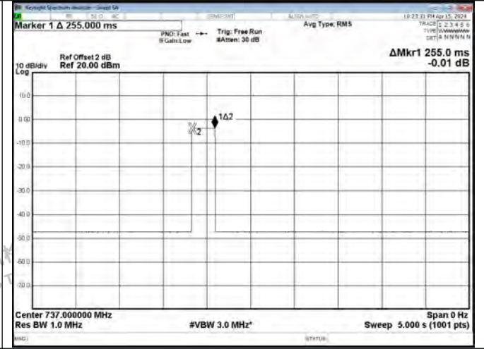
Detection Time-Lower 700 Band DL
