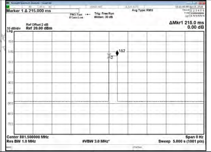
Detection Time-Cellular Band DL
