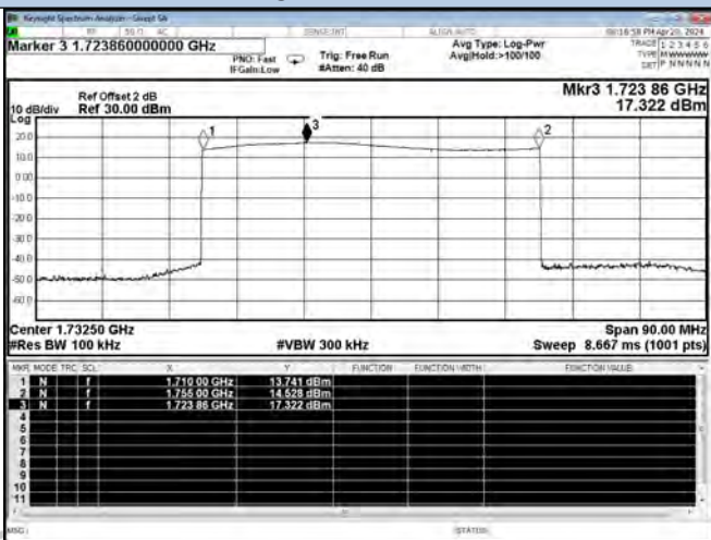
AWS Band
