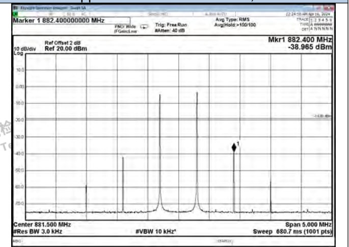
Cellular Band AGC+10dB, DL
