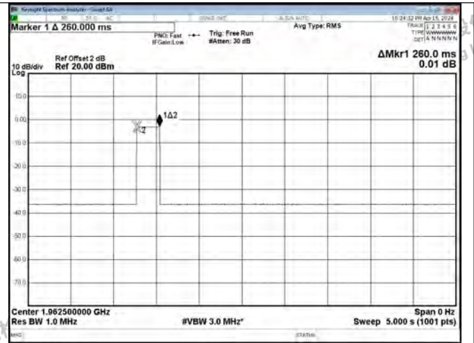
Detection Time-PCS Band DL
