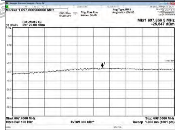
Lower 700 Band UL-CDMA Left Side Pre AGC
