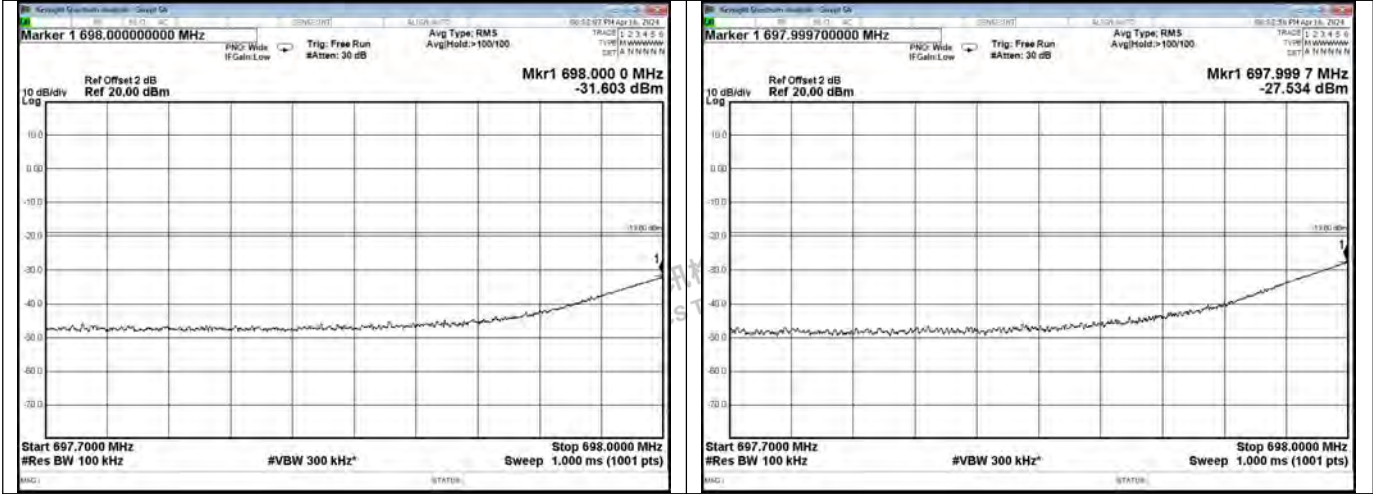
Lower 700 Band UL-GSM Left Side Pre AGC
