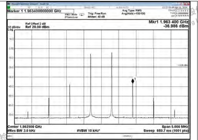
PCS Band AGC+10dB, DL
