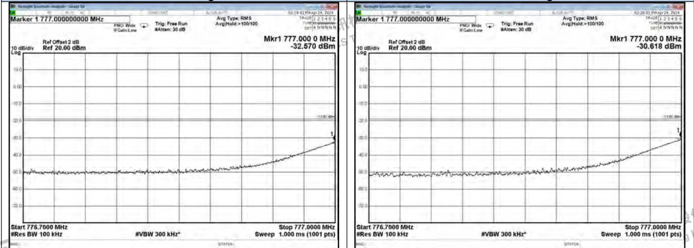
Upper 700 Band UL-GSM Left Side Pre AGC
