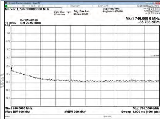
Lower 700 Band DL-GSM Right Side Pre AGC
