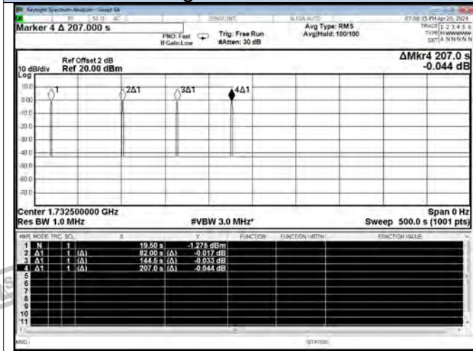
Restarting Time-AWS Band UL
