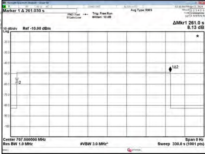
Lower 700 Band
