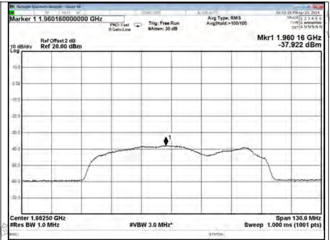
PCS Band DL
