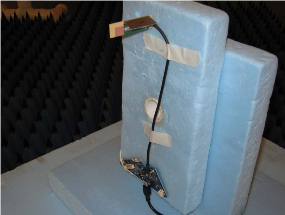
Radiated Emissions – Y Position (5)
