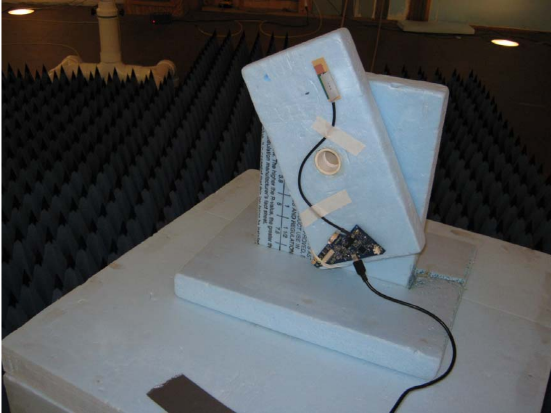
Radiated Emissions – Y – Worst Case Position
