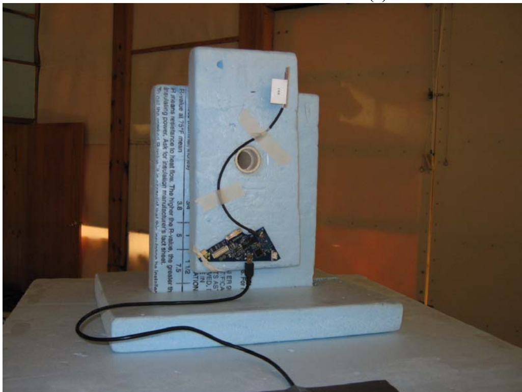
Radiated Emissions – Y Position (2)
