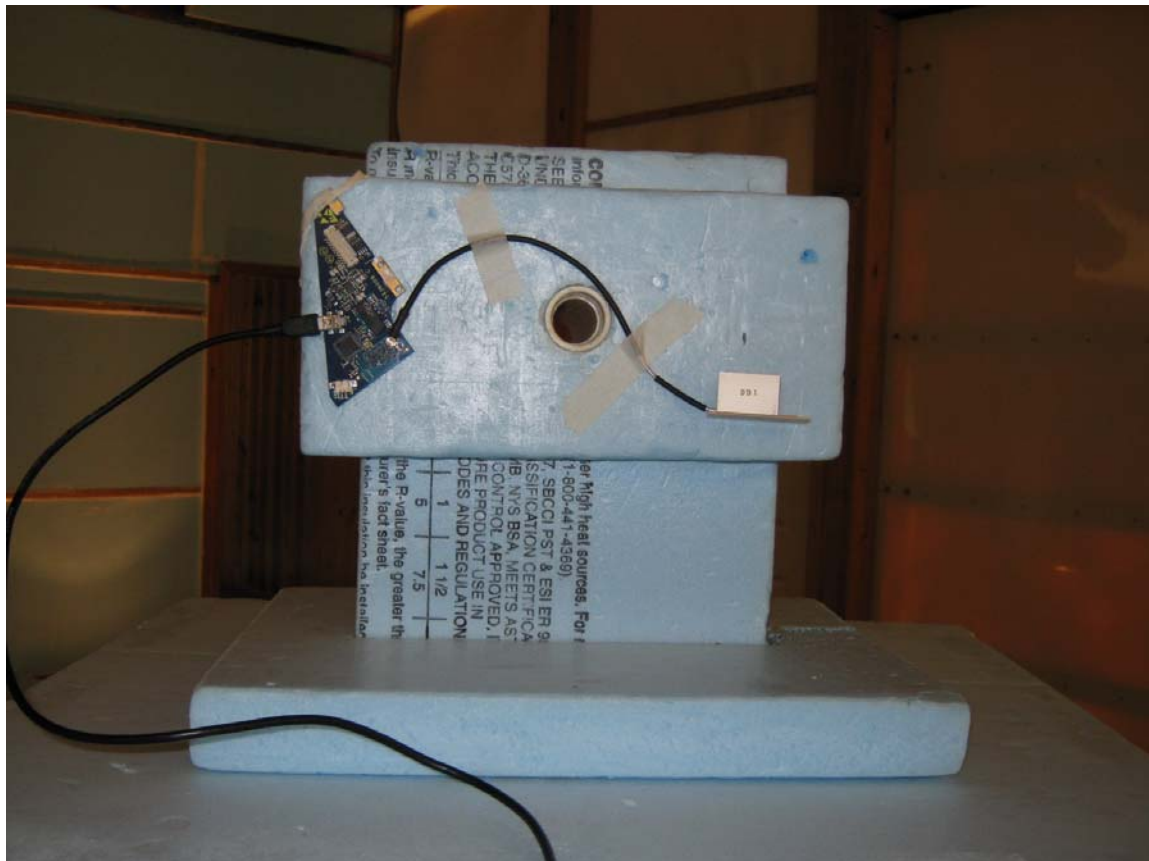
Radiated Emissions – X Position
