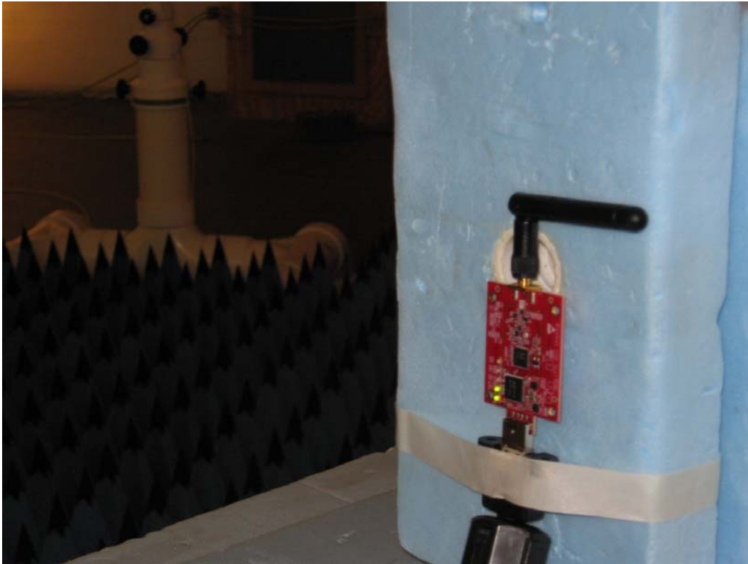
Radiated Emissions – Y – Worst Case Position
