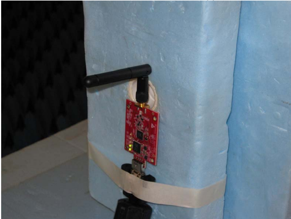
Radiated Emissions – Y Position (3)
