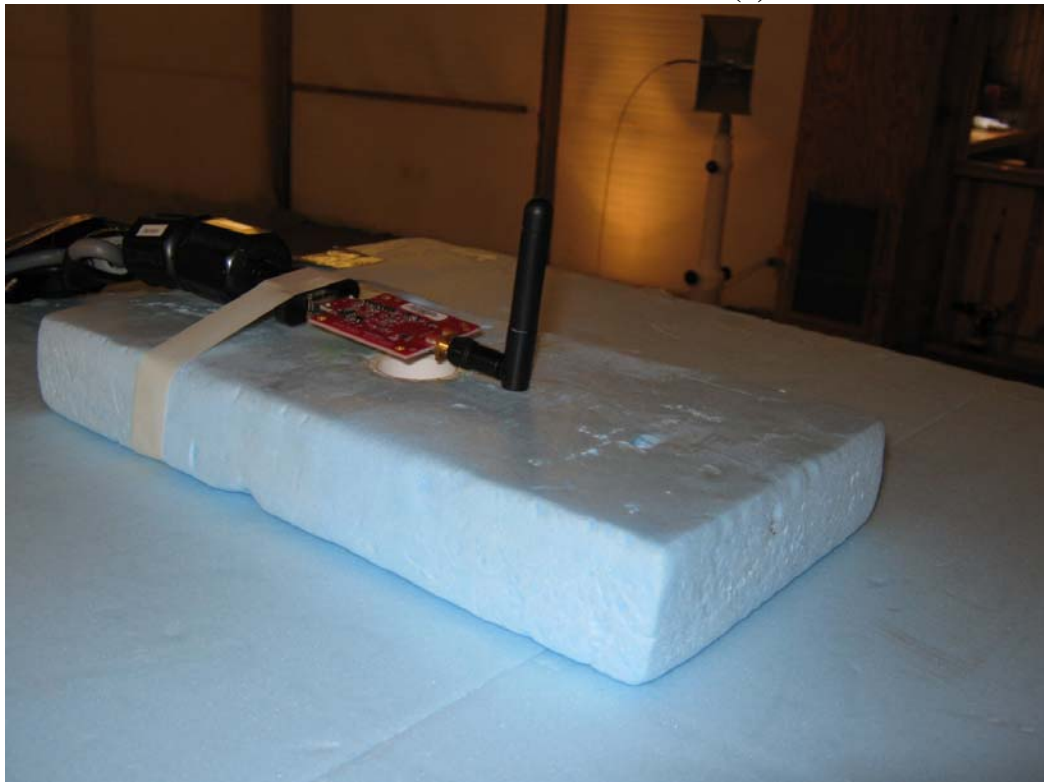
Radiated Emissions – Z Position (3)
