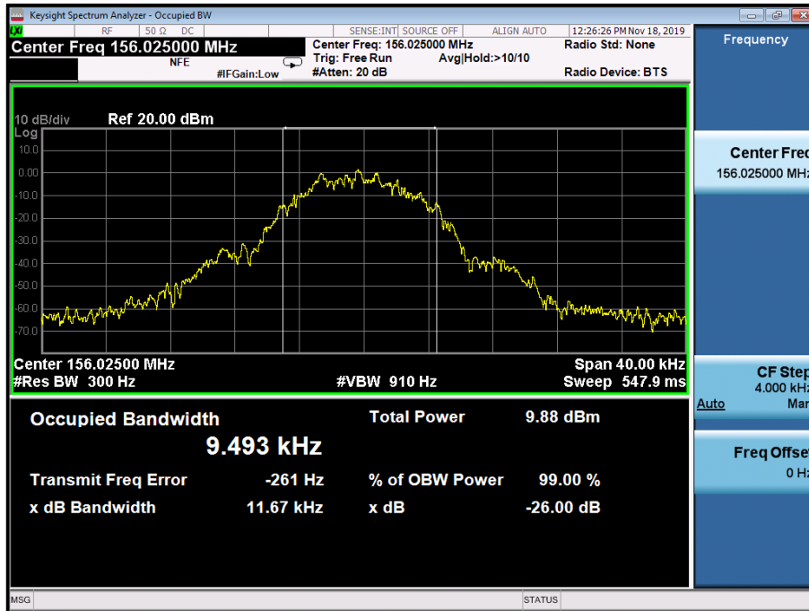
Figure 3 - 156.025 MHz Occupied Bandwidth
