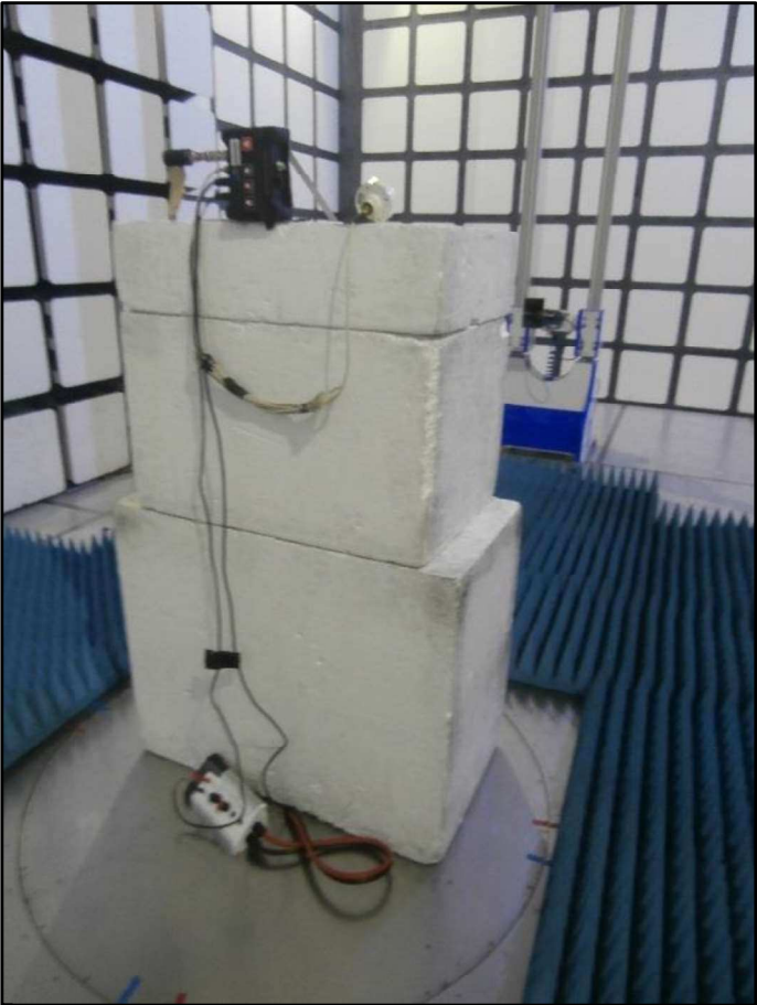
Figure 58 –1 GHz to 2 GHz, EUT Orientation Z
