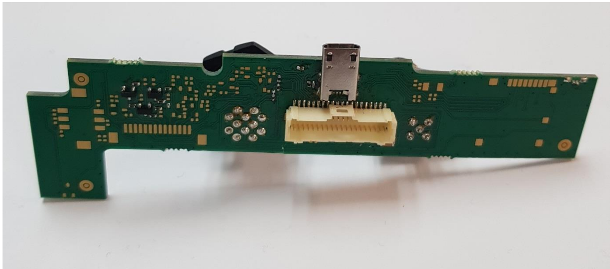
Fig 9: B500 Connector Board Back
