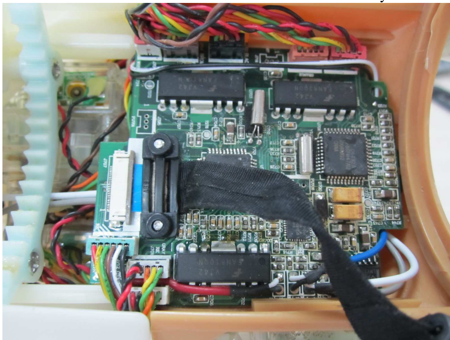
The PCB that controlled the action of the rear body
