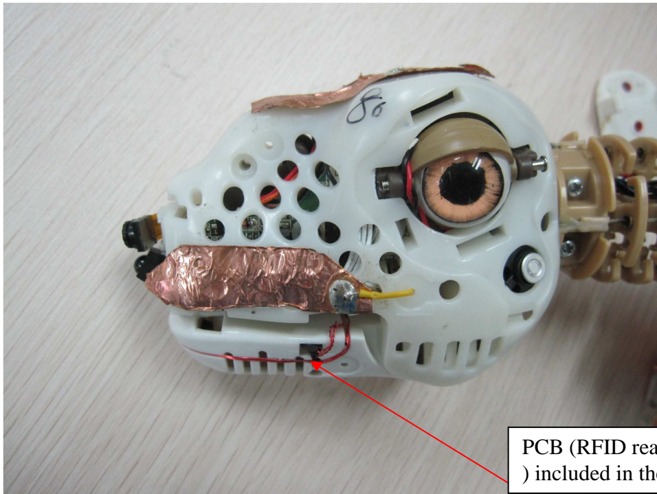
Head view RFID reader included
