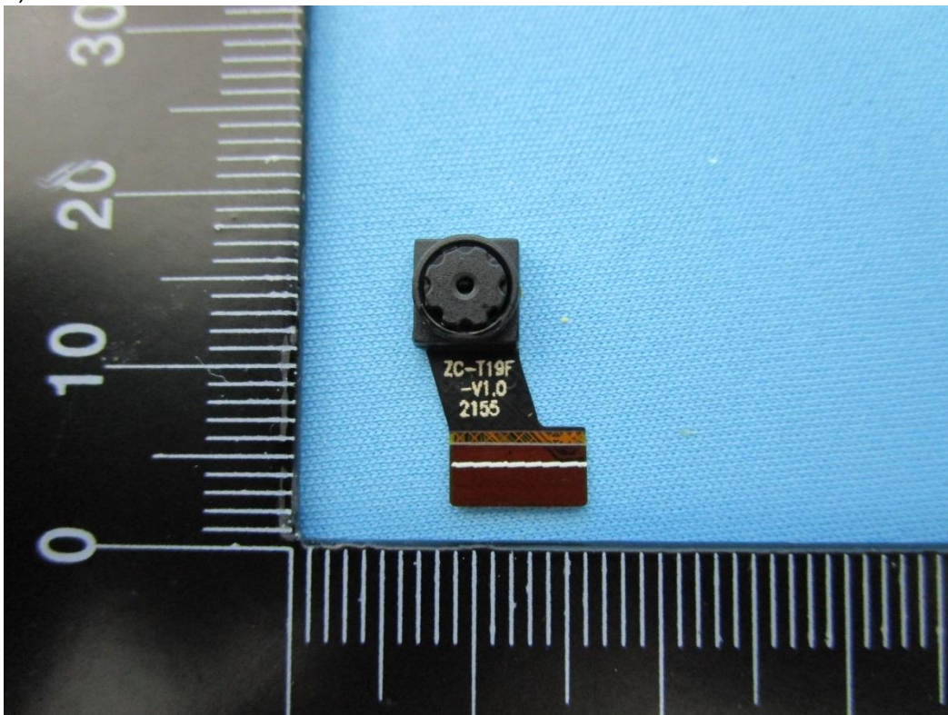
(26) EUT Photo
