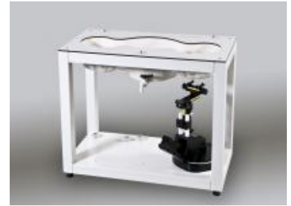
Figure 3.6 SAM Twin Phantom
