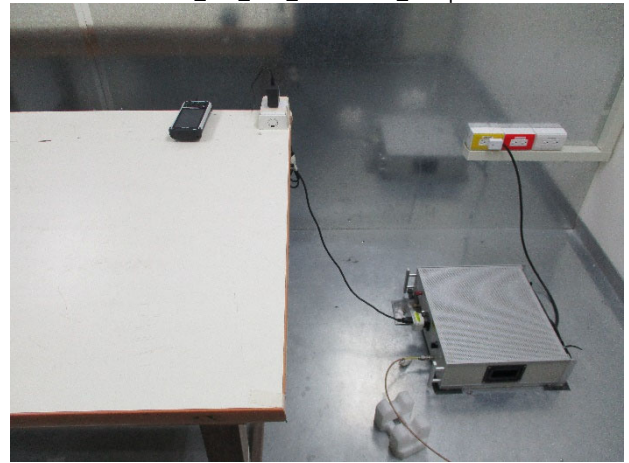
15_247_BLE_Conduction_Setup
