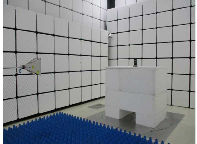
15_247_WLAN_Radiated_Setup
