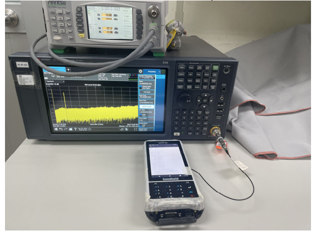
15_407_Radiated_Setup
