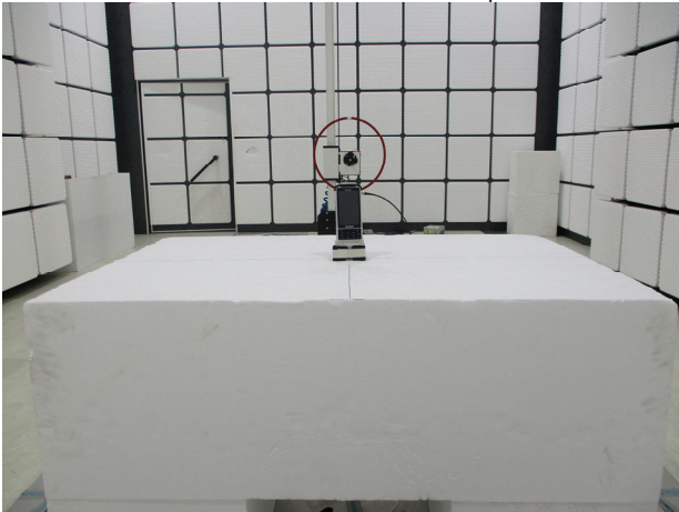
15_247_WLAN_Radiated_Setup
