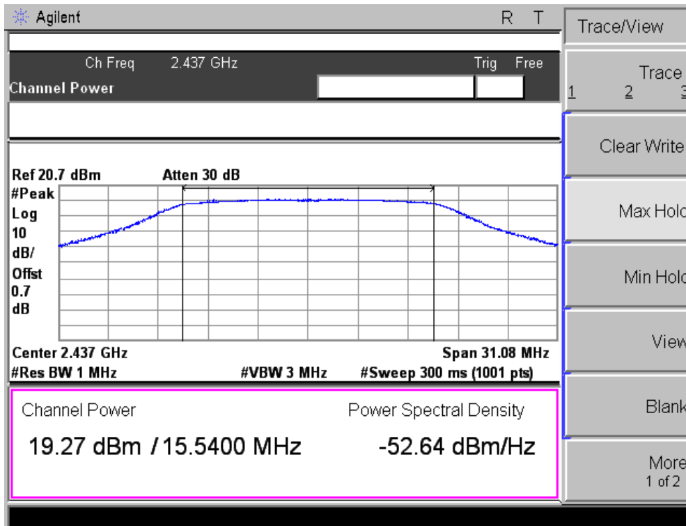
– 802.11n 6CH (Peak Power)–
