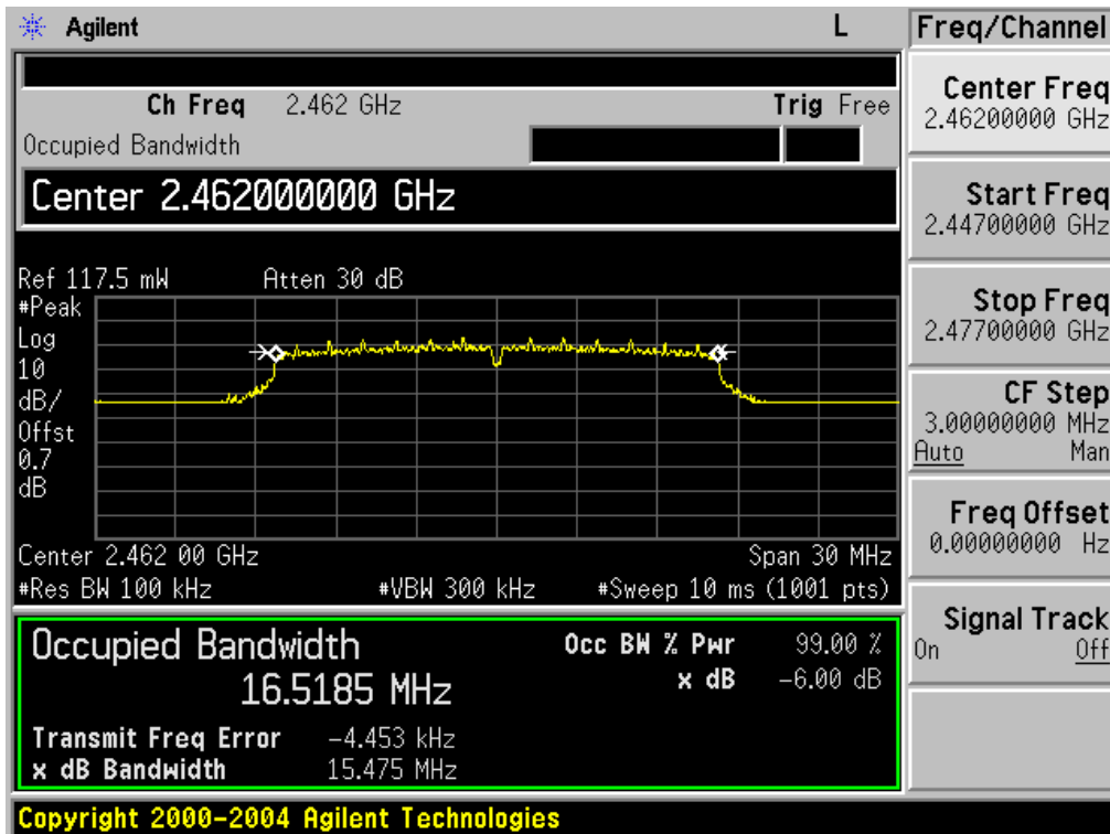
- 802.11g 11CH -
