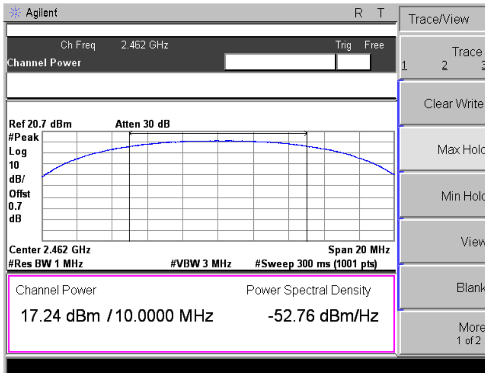
- 802.11b 11CH (Peak Power)-
