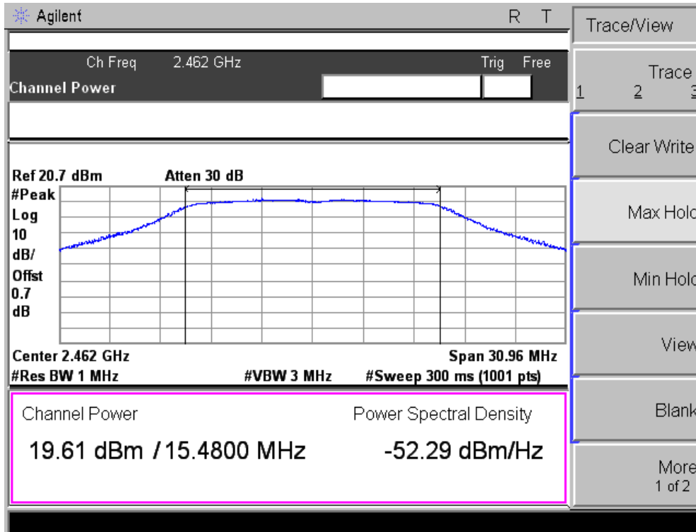
- 802.11g 11CH (Peak Power)-
