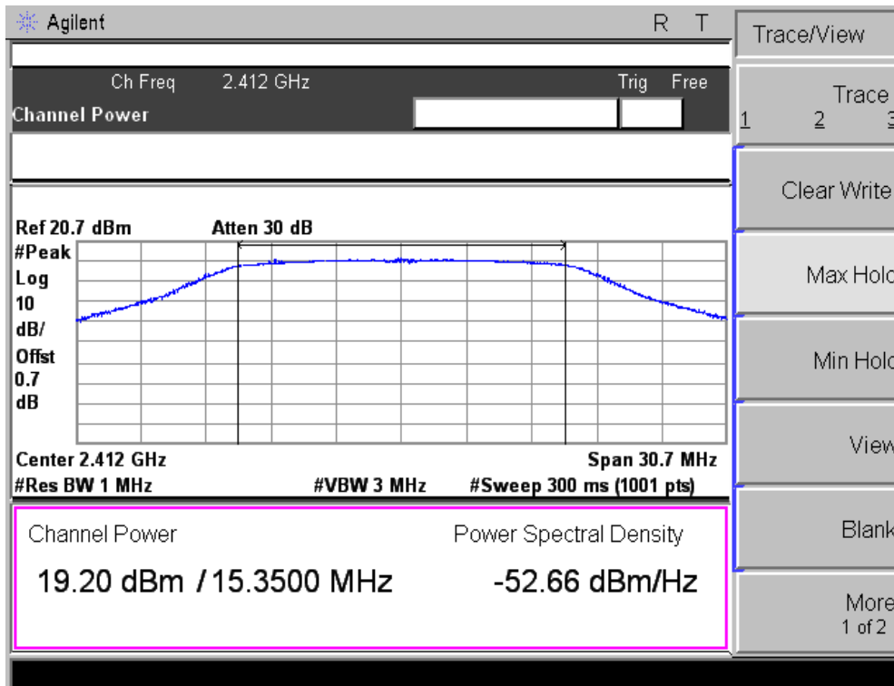
– 802.11n 1CH (Peak Power)–
