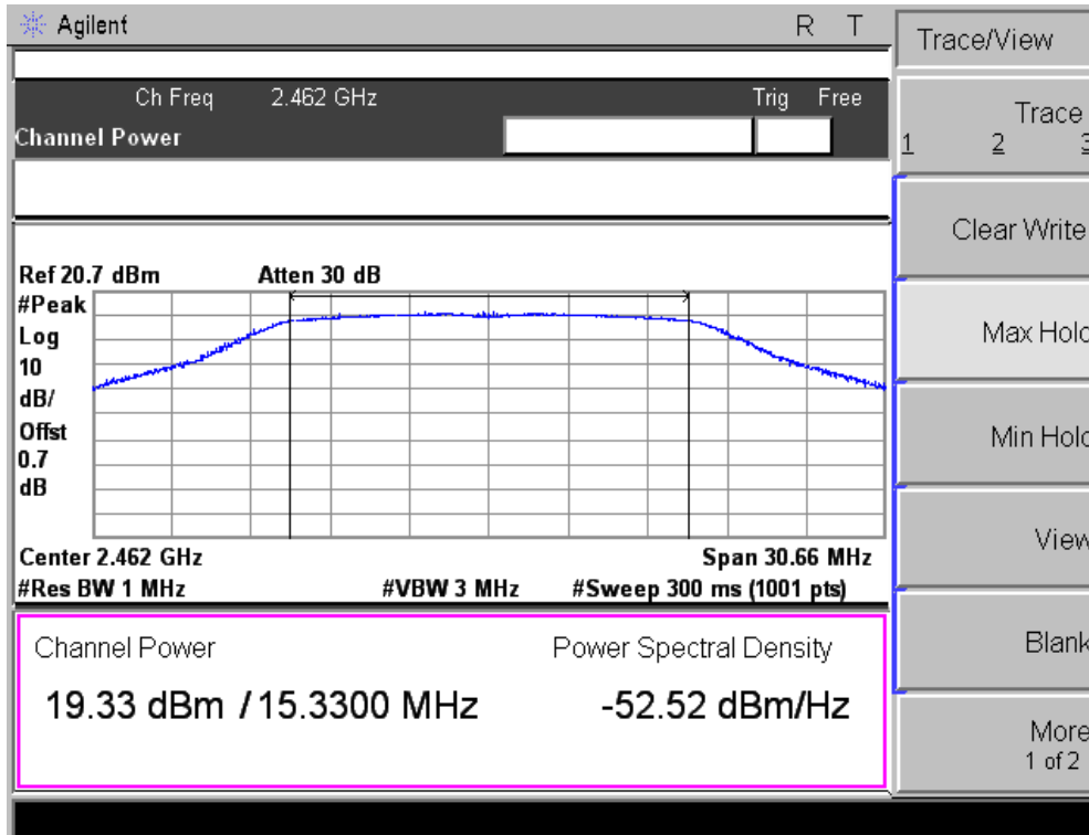
- 802.11n 11CH (Peak Power)-
