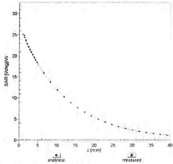
f = 1750 MHz, WGLS R22 (H_convF)
