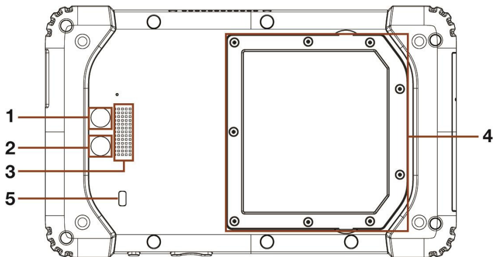
FIGURE 2.3. BACK PANEL
