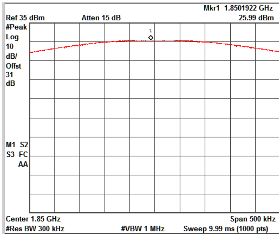
GSM_E-GPRS_Channel No. 512
