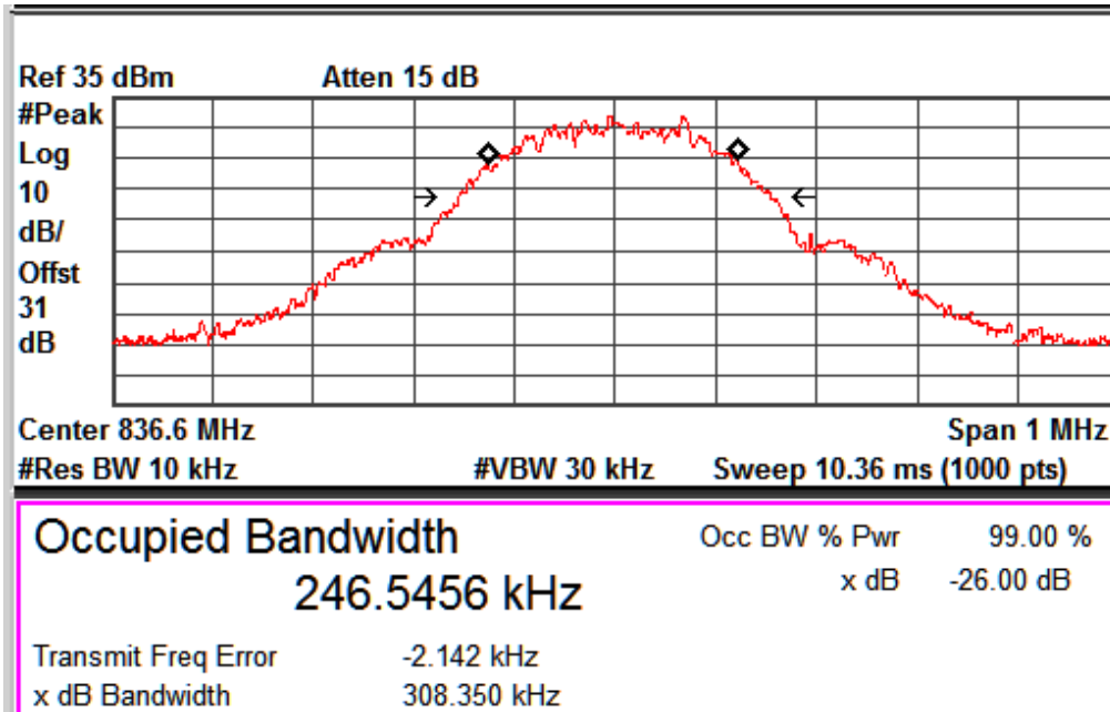
GSM_GPRS_Channel No. 190
