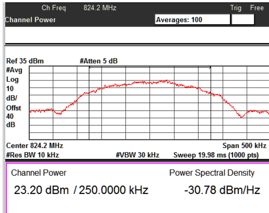
GSM_E-GPRS_Channel No. 128
