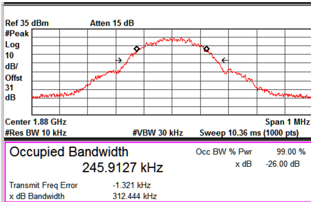
GSM_GPRS_Channel No. 661
