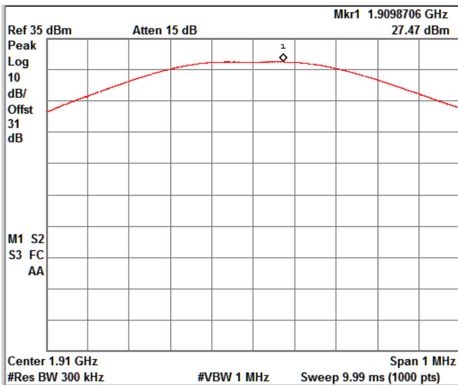
GSM_Voice_Channel No. 810
