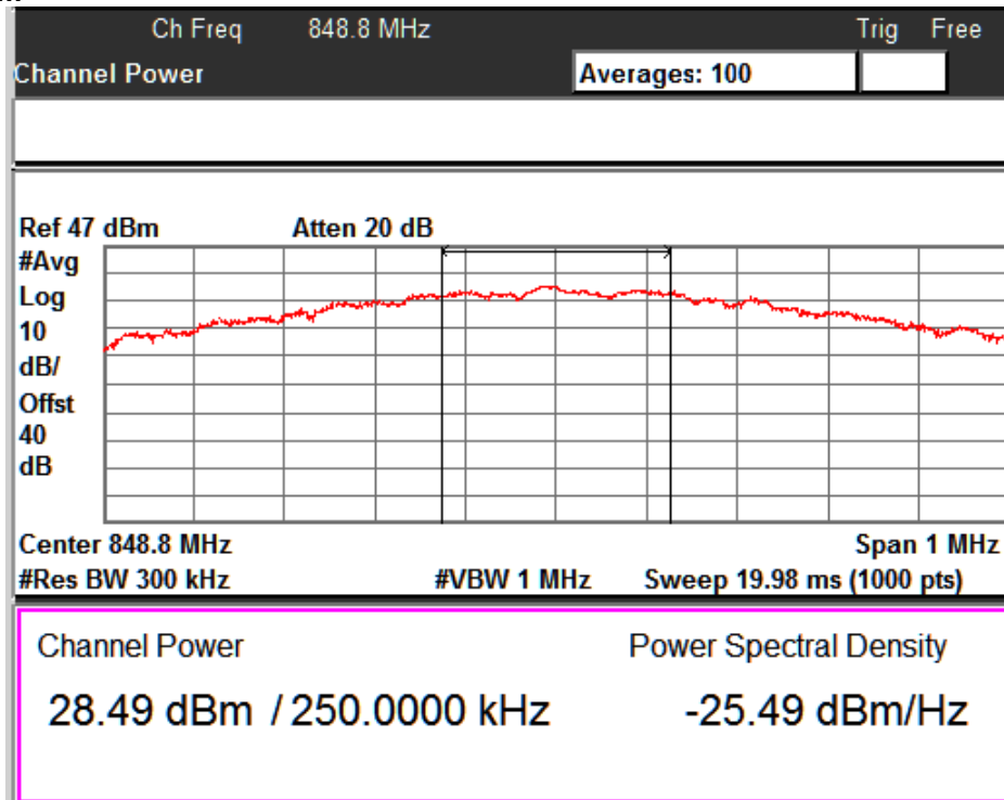
GSM_GPRS_Channel No. 251
