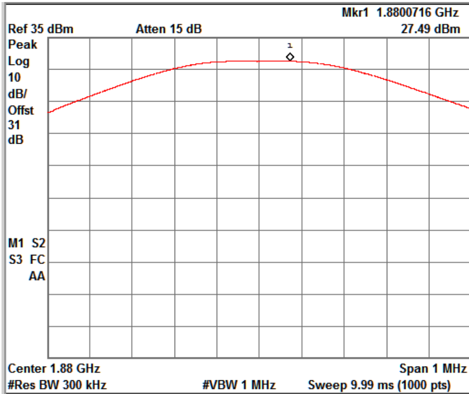
GSM_Voice_Channel No. 661
