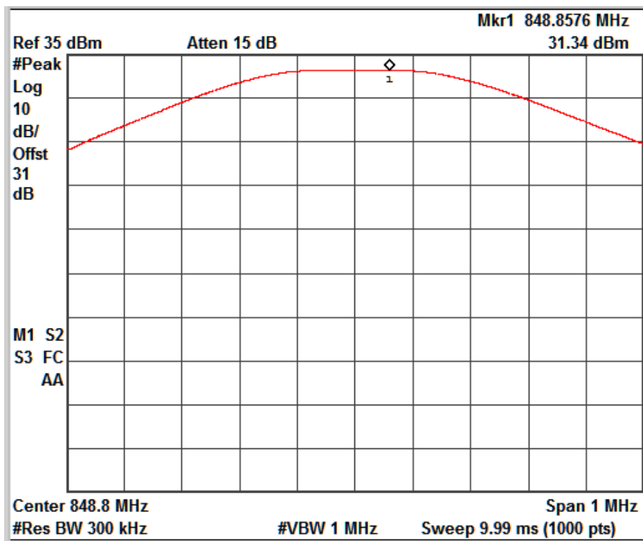
GSM_GPRS_Channel No. 251
