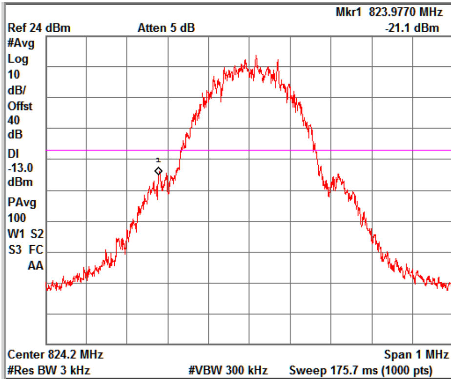
GSM_Voice_Channel No. 128
