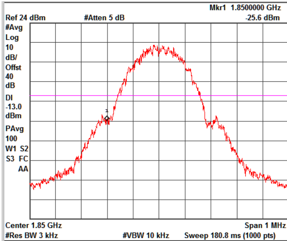
GSM_GPRS_Channel No. 512
