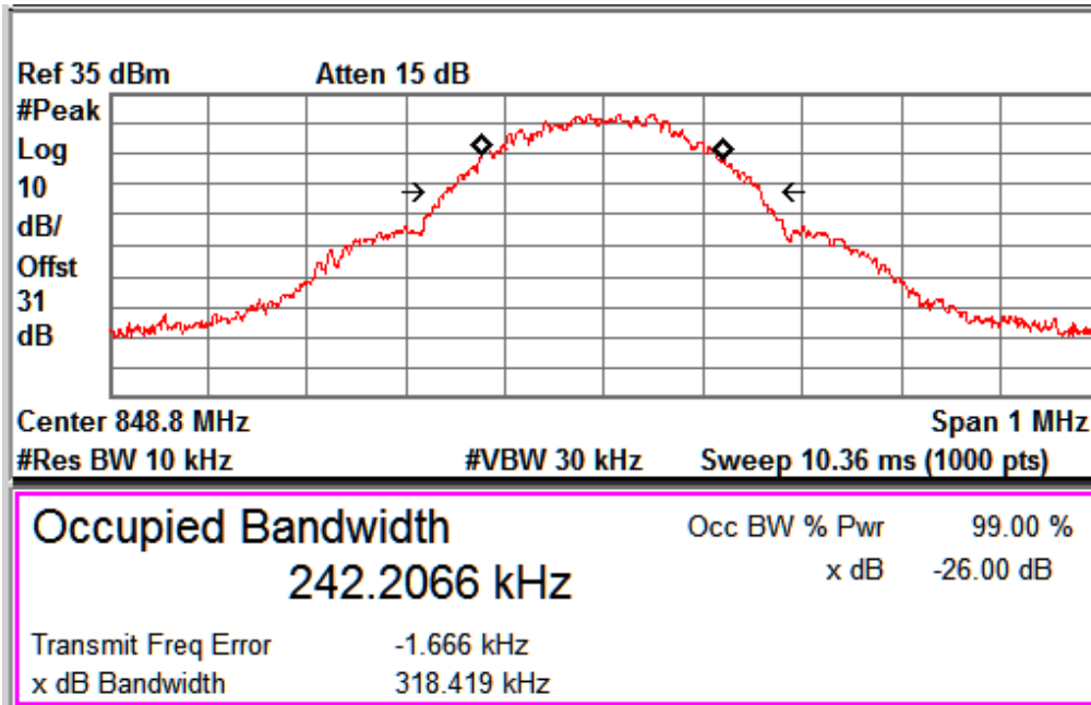
GSM_Voice_Channel No. 251
