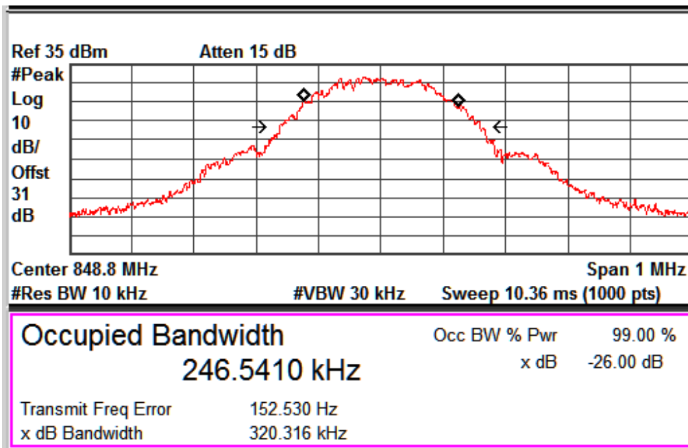
GSM_GPRS_Channel No. 251
