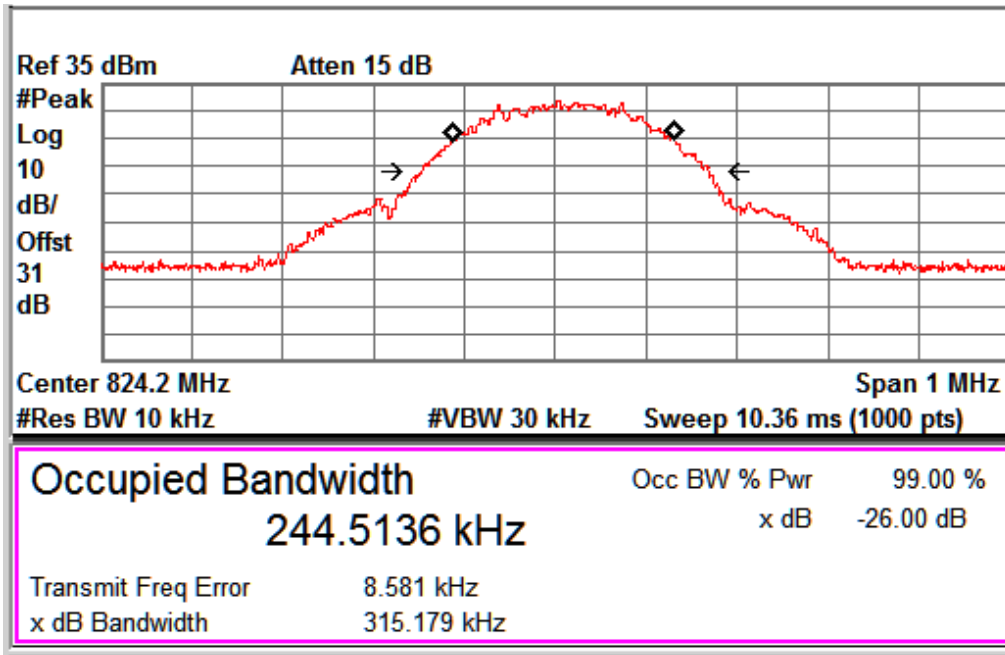
GSM_Voice_Channel No. 128
