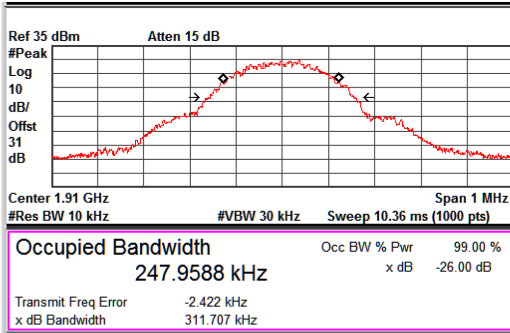
GSM_GPRS_Channel No. 810
