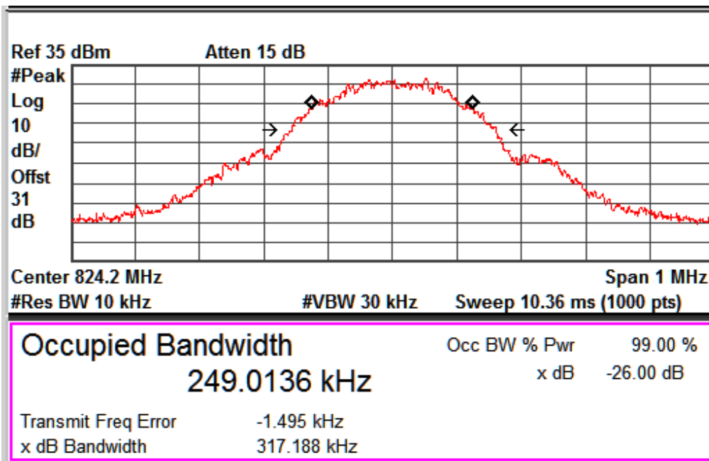
GSM_GPRS_Channel No. 128
