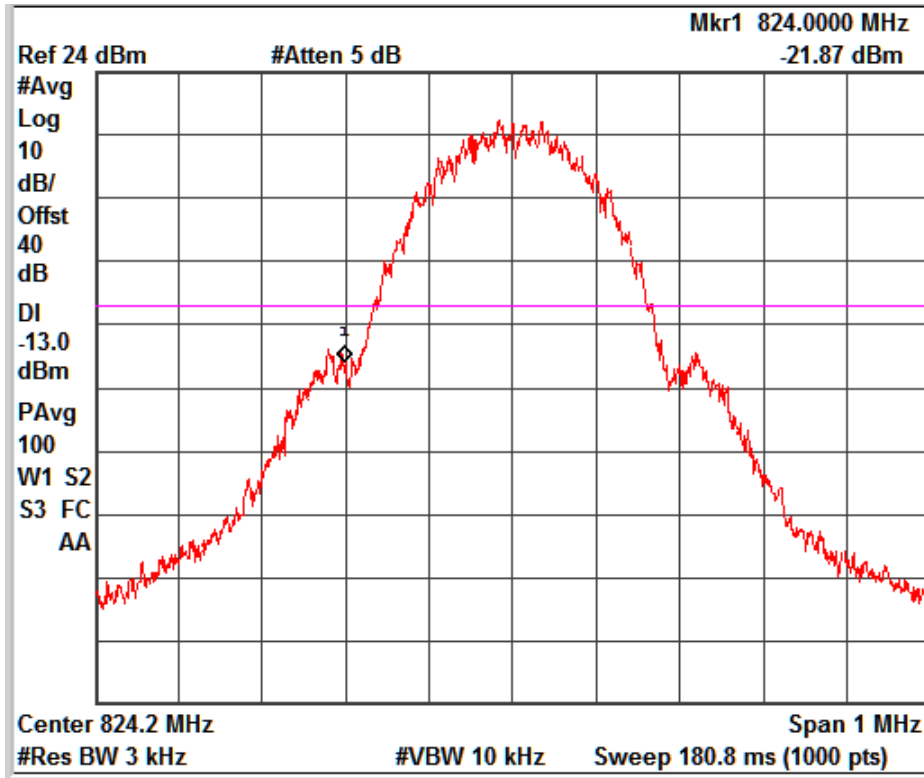
GSM_GPRS_Channel No. 128
