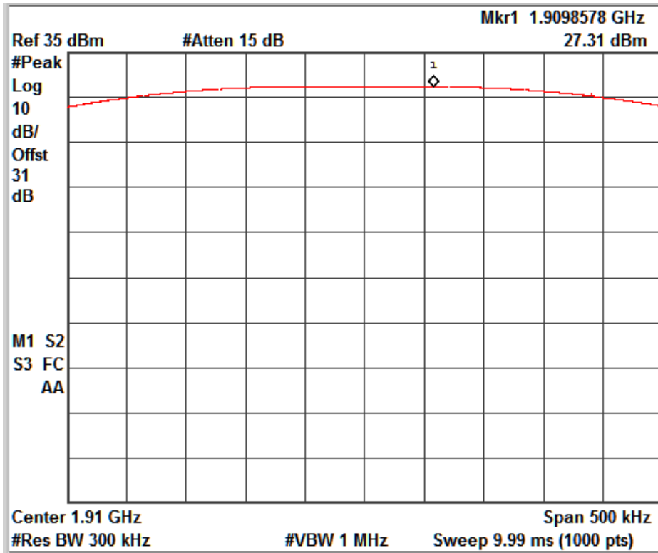
GSM_GPRS_Channel No. 810
