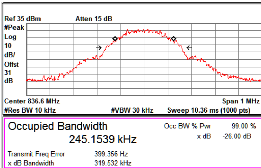
GSM_Voice_Channel No. 190
