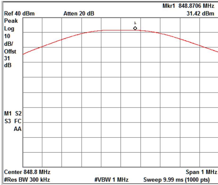
GSM_Voice_Channel No. 251
