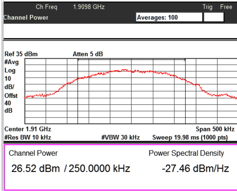
GSM_Voice_Channel No. 810
