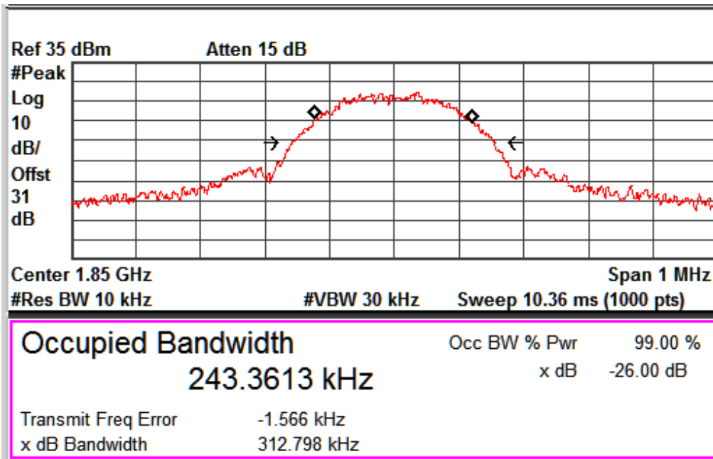
GSM_E-GPRS_Channel No. 512
