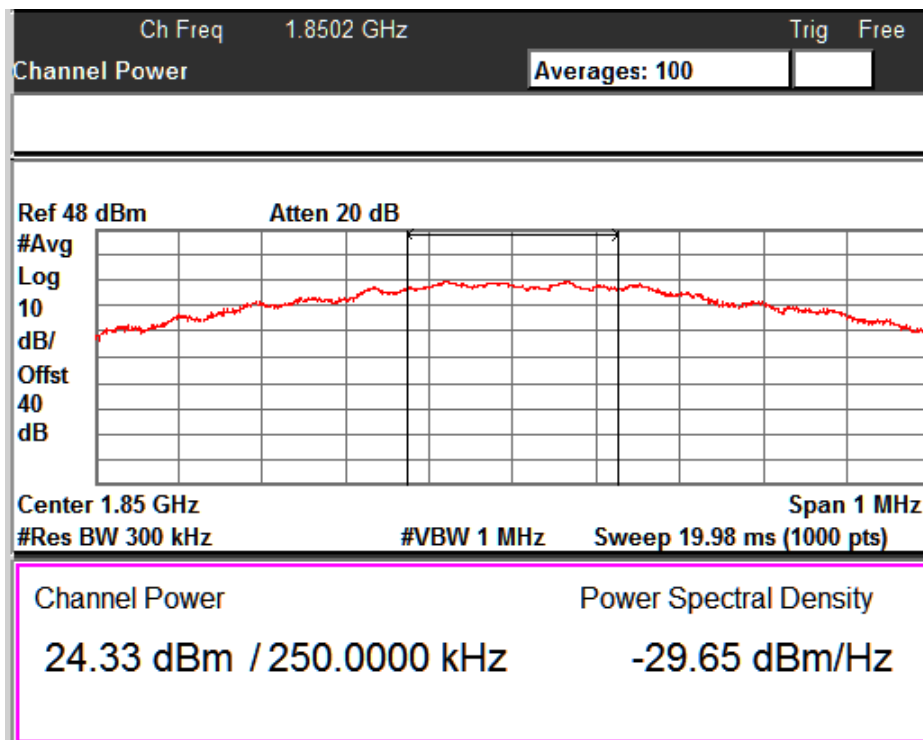
GSM_GPRS_Channel No. 512
