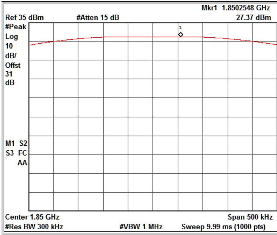
GSM_GPRS_Channel No. 512
