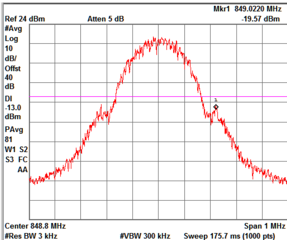
GSM_Voice_Channel No. 251
