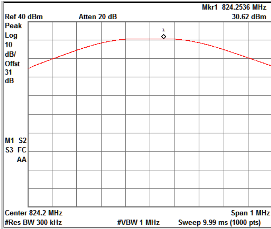
GSM_Voice_Channel No. 128
