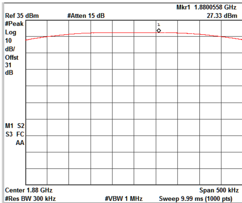
GSM_GPRS_Channel No. 661
