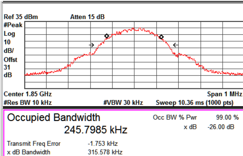
GSM_GPRS_Channel No. 512
