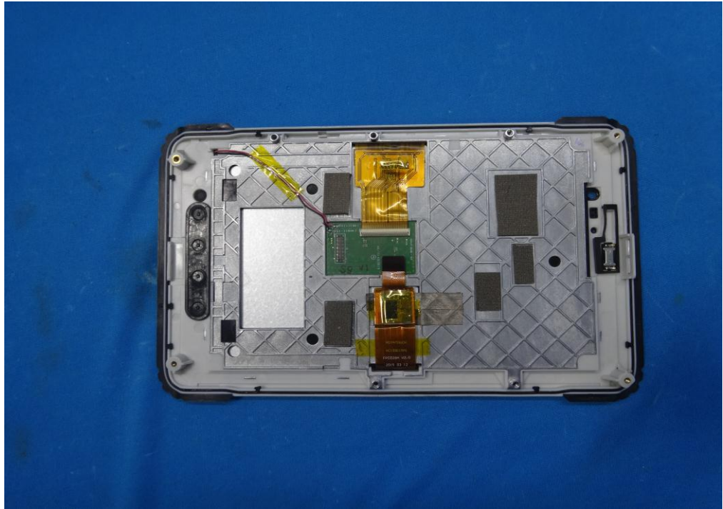
Outside Panel removed
