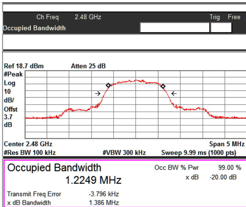
99% Occupied Bandwidth: Channel High
