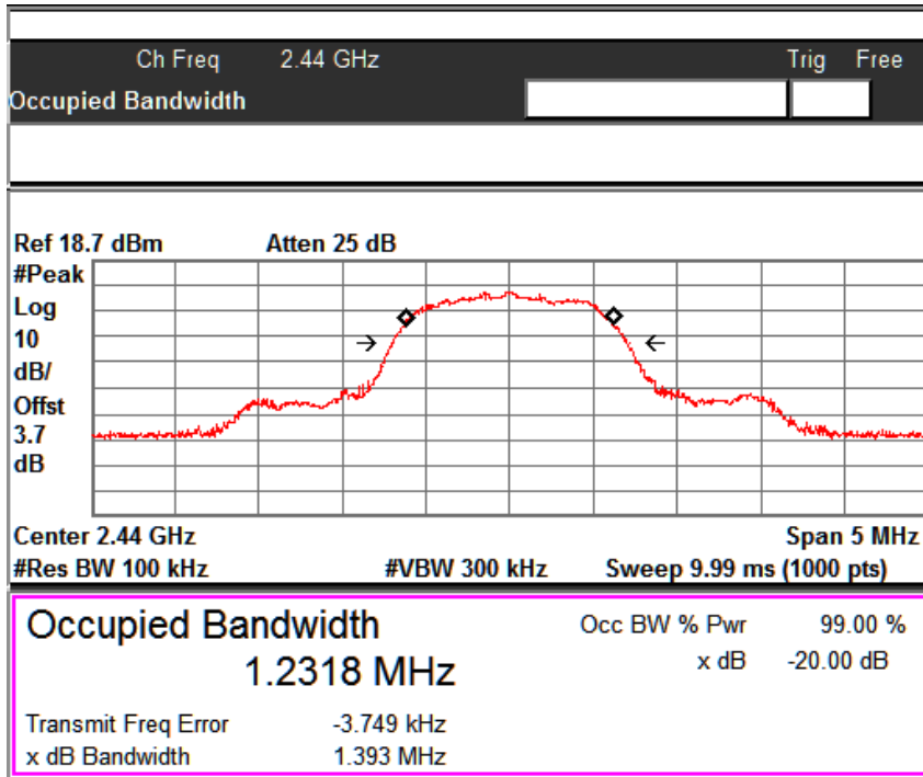
99% Occupied Bandwidth: Channel Mid
