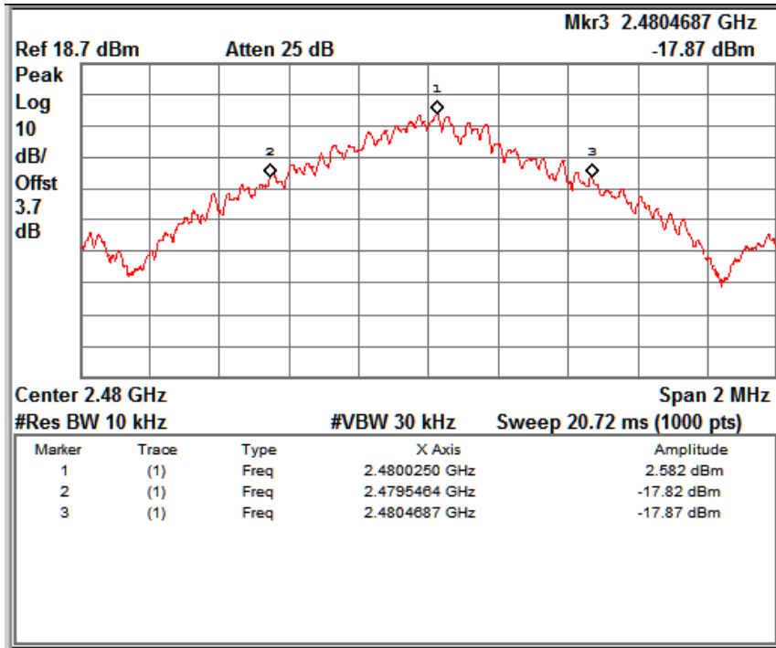
Channel High: 20dB Bandwidth Measurement
