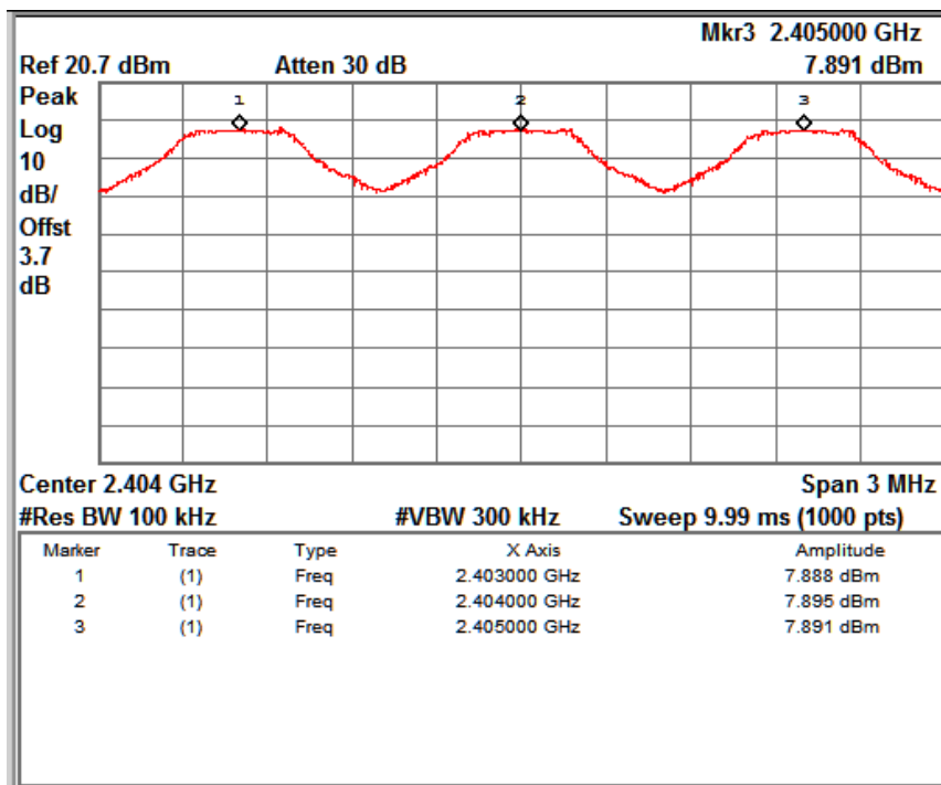
Channel Separation
