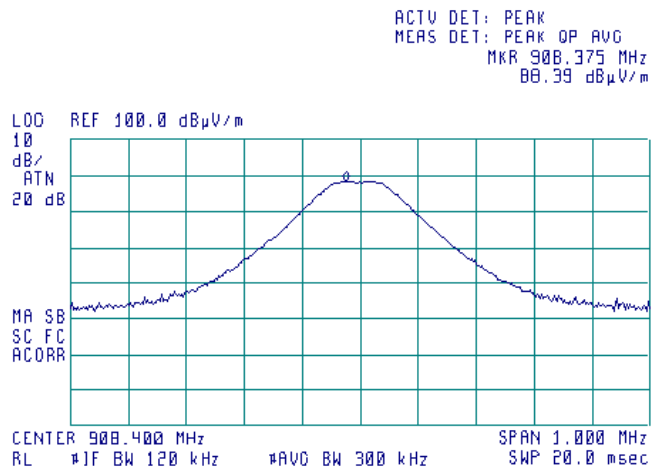
Plot 7.1.10 Radiated emission measurements at the fundamental frequency
