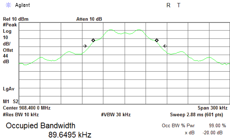
Plot 7.2.1 Occupied bandwidth test result
