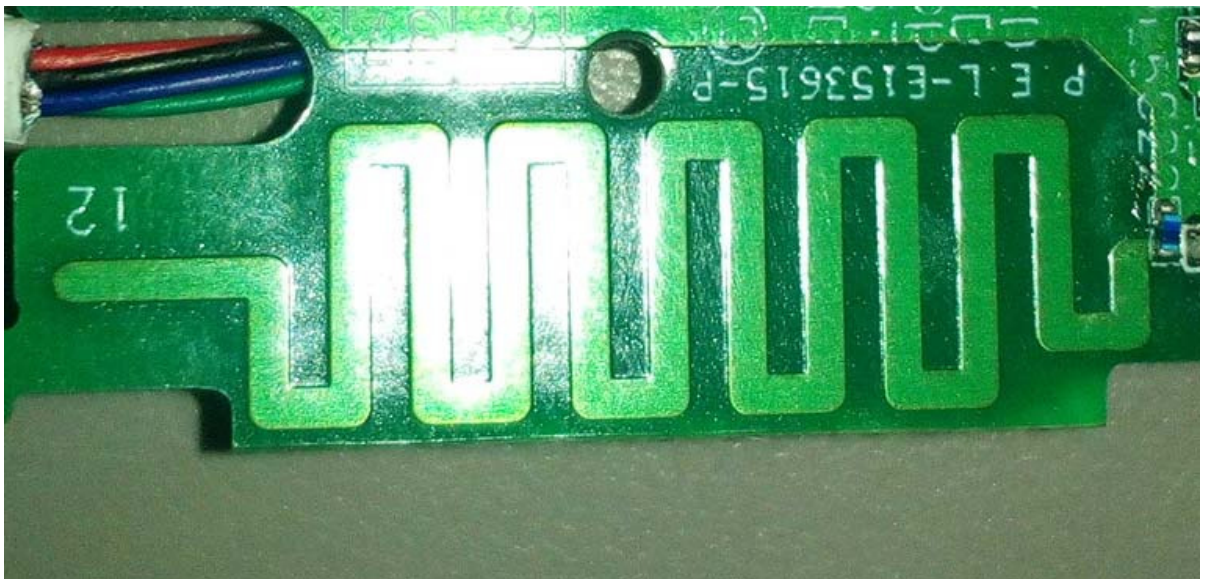
Photograph 7.5.1 Antenna assembly
