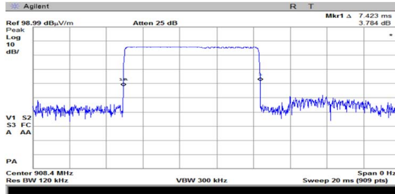
Plot 7.2.13 Transmission pulse period
