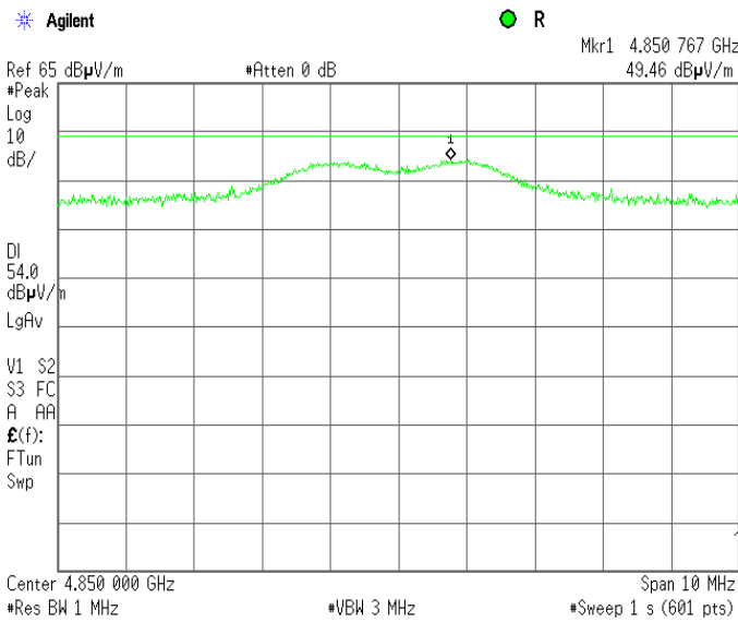
Plot 7.3.10 Radiated emission measurements at the third harmonic of carrier frequency
