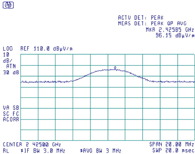
Plot 7.2.6 Field strength of carrier in horizontal antenna polarization, Z-axis position
