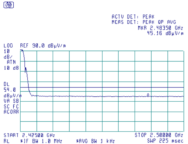
Plot 7.4.2 The highest emission level at 2483.5 MHz
