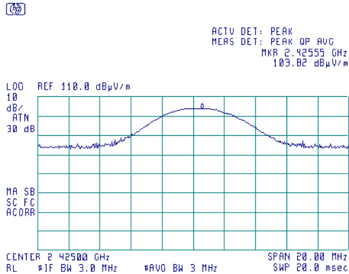
Plot 7.2.2 Field strength of carrier in horizontal antenna polarization, X-axis position
