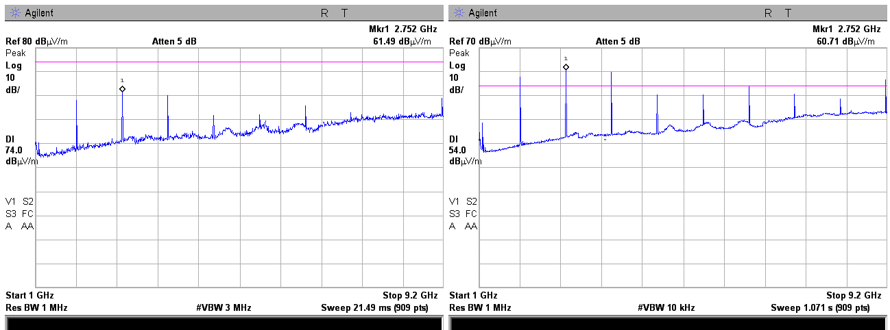
Plot 7.2.8 Radiated emission measurements from 1000 to 9200 MHz
