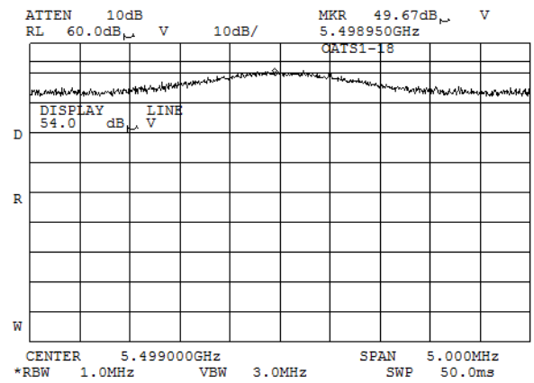
Plot 7.2.15 Radiated emission measurements at the sixth harmonic frequency
