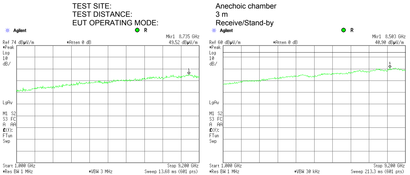
Plot 8.1.4 Radiated emission measurements in 1000 – 9200 MHz, horizontal antenna polarization
