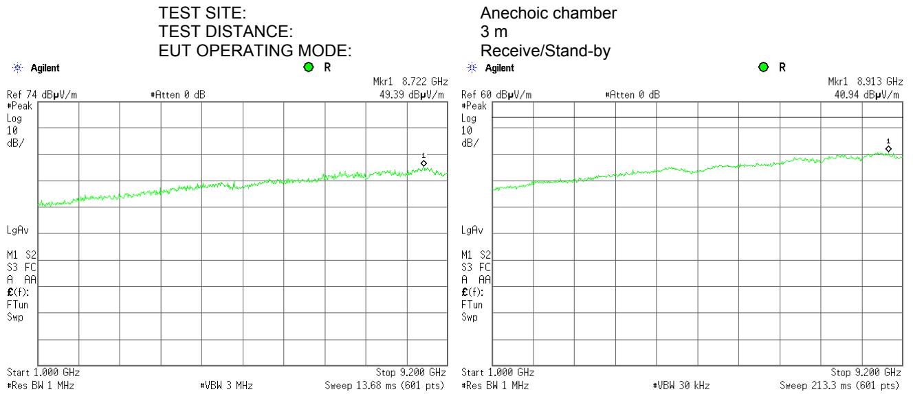
Plot 8.1.3 Radiated emission measurements in 1000 – 9200 MHz, vertical antenna polarization
