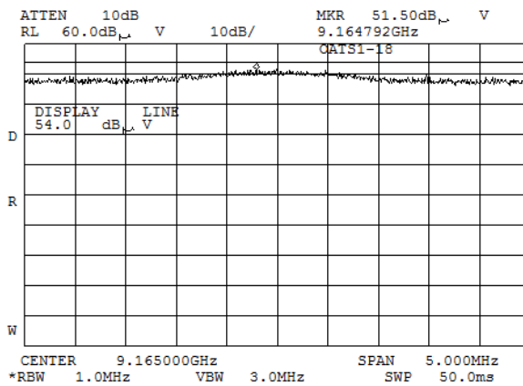
Plot 7.2.17 Radiated emission measurements at the tenth harmonic frequency
