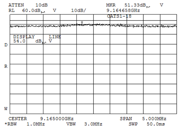
Plot 7.2.17 Radiated emission measurements at the tenth harmonic frequency
