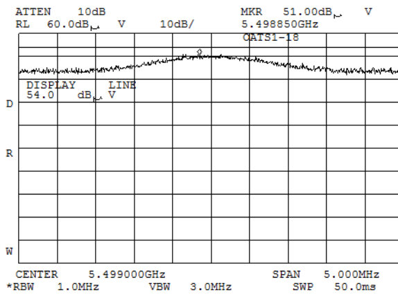
Plot 7.2.15 Radiated emission measurements at the sixth harmonic frequency
