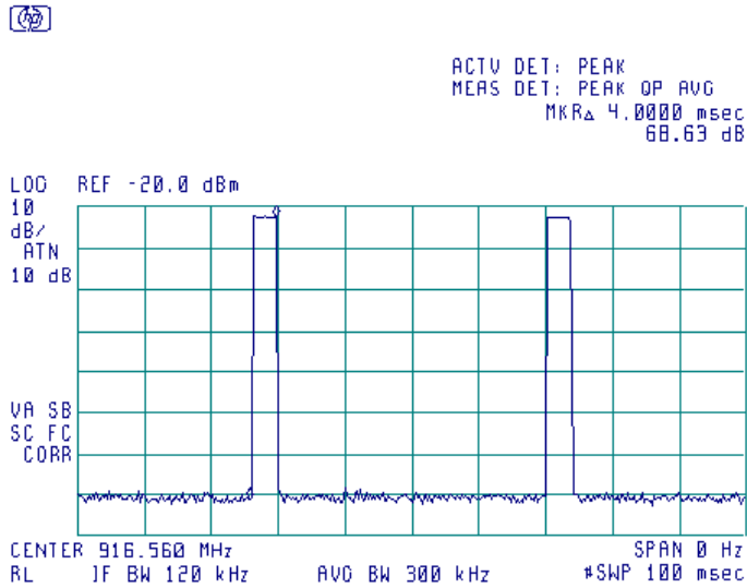
Plot 7.2.19 Transmission pulse period
