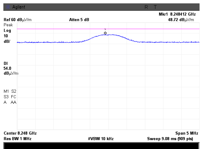
Plot 7.2.23 Radiated emission measurements at the 9th harmonic frequency
