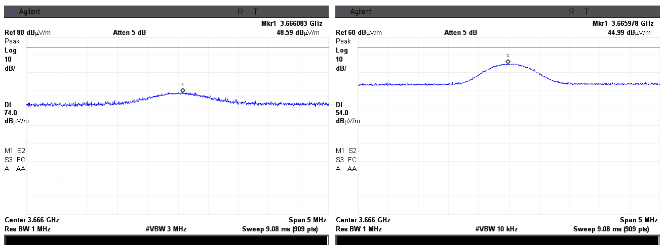
Plot 7.2.13 Radiated emission measurements at the fourth harmonic frequency
