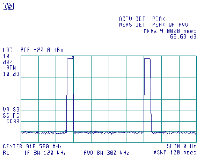
Plot 7.2.27 Transmission pulse period
