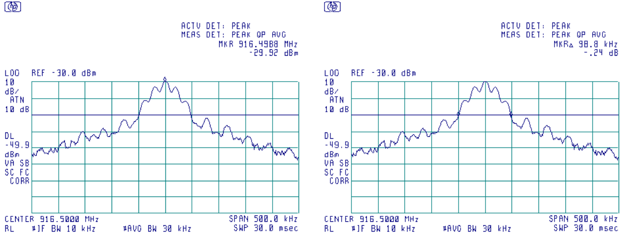
Plot 7.3.2 Occupied bandwidth test result, 99% power
