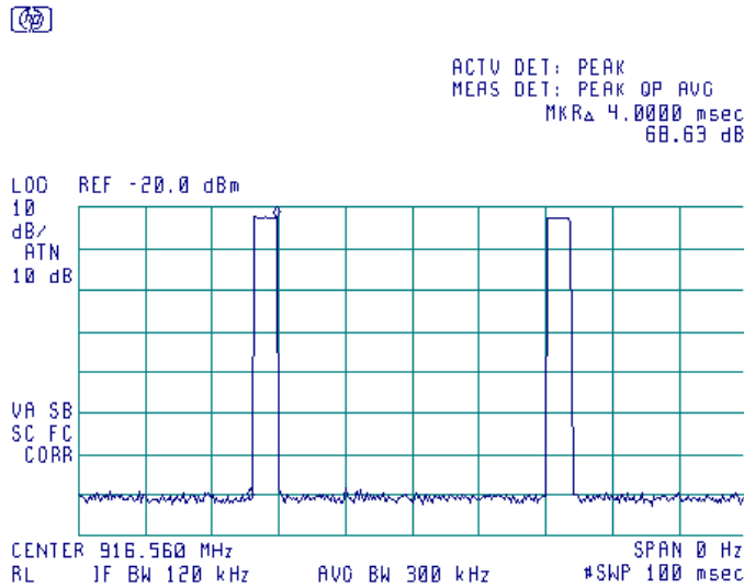
Plot 7.2.22 Transmission pulse period
