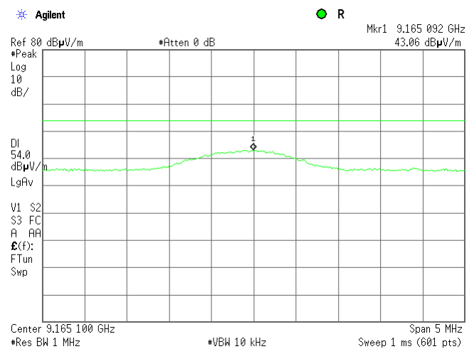
Plot 7.2.20 Radiated emission measurements at the 10 th harmonic frequency
