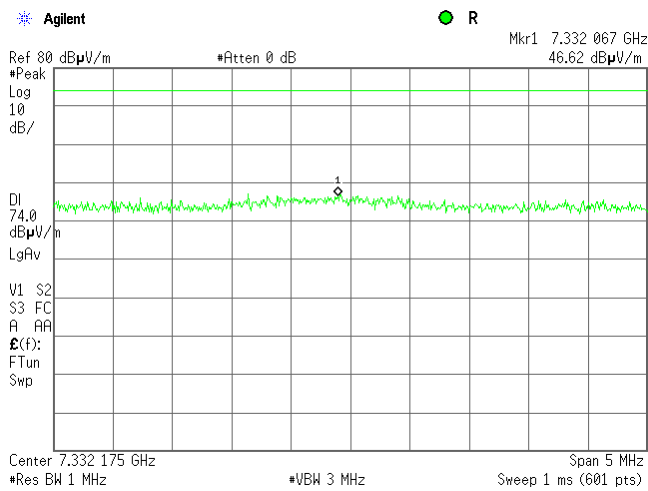
Plot 7.2.18 Radiated emission measurements at the 8 th harmonic frequency
