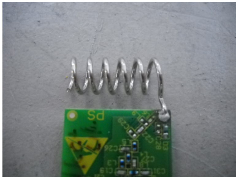
Photograph 7.4.1 Antenna assembly
