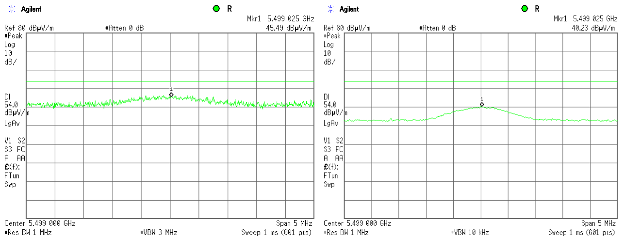
Plot 7.2.16 Radiated emission measurements at the six harmonic frequency
