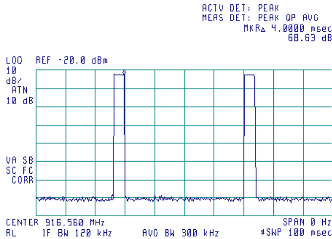
Plot 7.1.3 Polling / supervision transmission period
