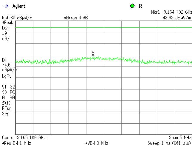
Plot 7.2.20 Radiated emission measurements at the 10 th harmonic frequency
