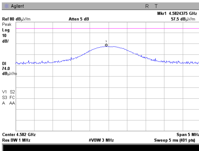
Plot 7.2.16 Radiated emission measurements at the fifth harmonic frequency
