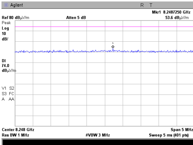
Plot 7.2.24 Radiated emission measurements at the ninth harmonic frequency
