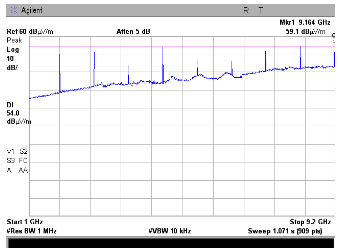
Plot 7.2.8 Radiated emission measurements from 1000 to 9200 MHz
