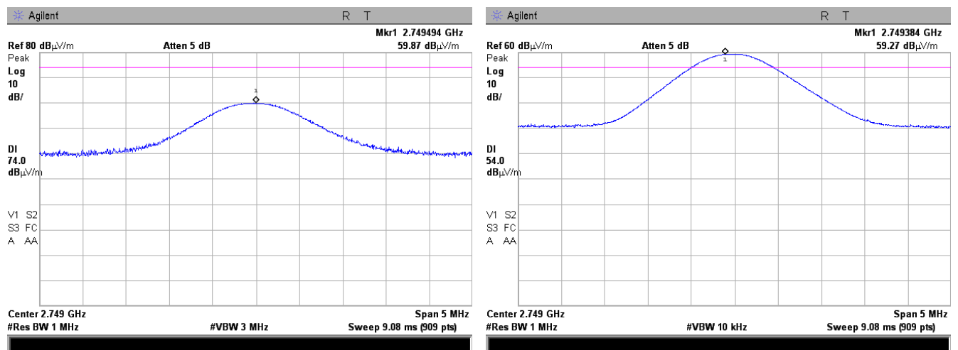
Plot 7.2.12 Radiated emission measurements at the third harmonic frequency
