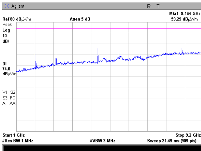
Plot 7.2.8 Radiated emission measurements from 1000 to 9200 MHz
