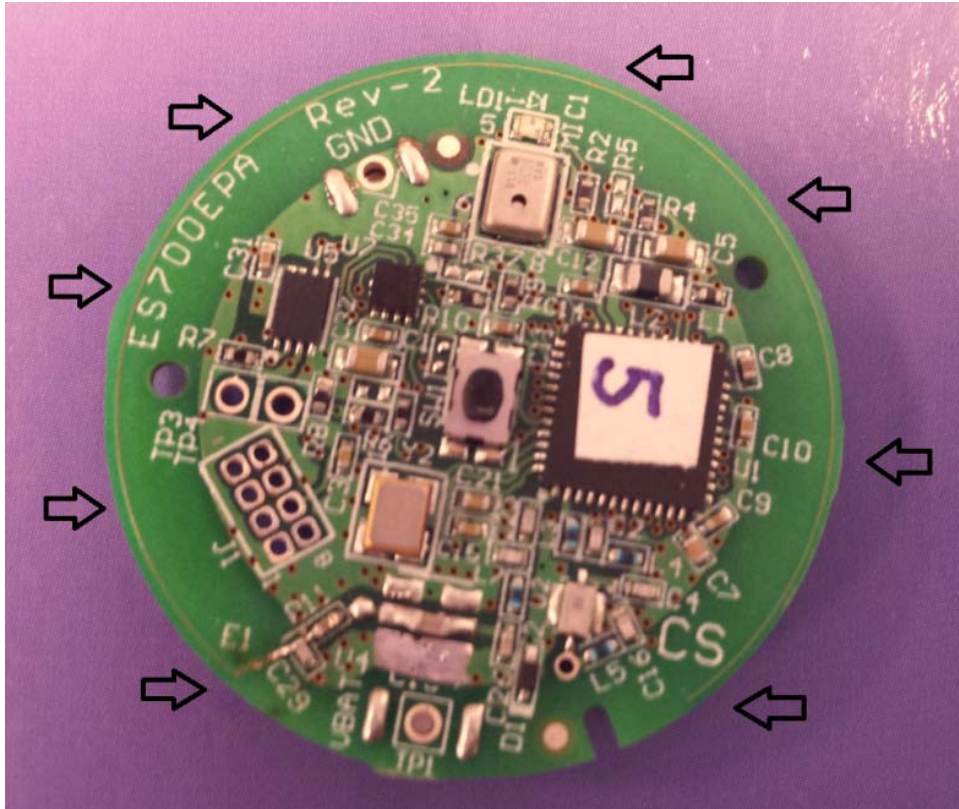
The antenna is printed, starts from point E1 on the left side and goes around the PCB
