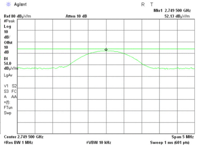
Plot 7.2.18 Radiated emission measurements at the third harmonic frequency
