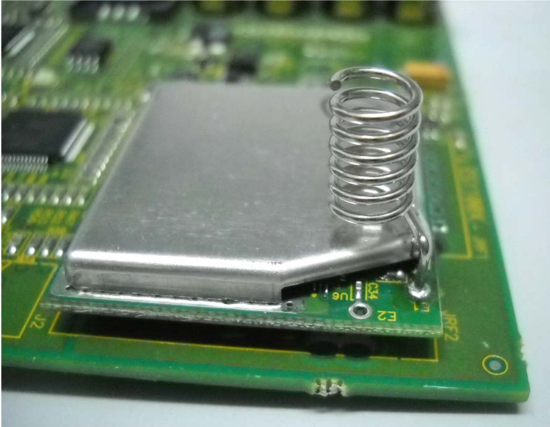
Photograph No.5 ES7000EG transceiver view
