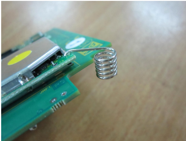
Photograph 7.5.1 Antenna assembly
