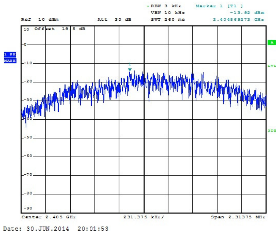
Figure 7.5.2-1: Power Spectral Density - Low Channel
