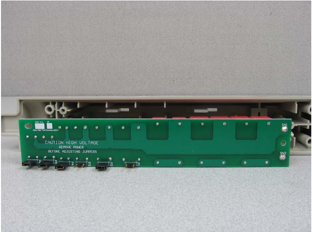
Figure 4: Internal Photo - High Voltage Board
