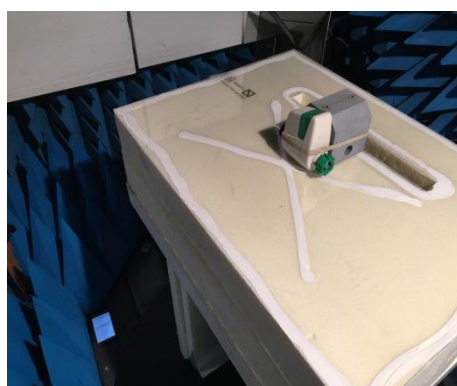
Test setup in anechoic chamber, axis Z
